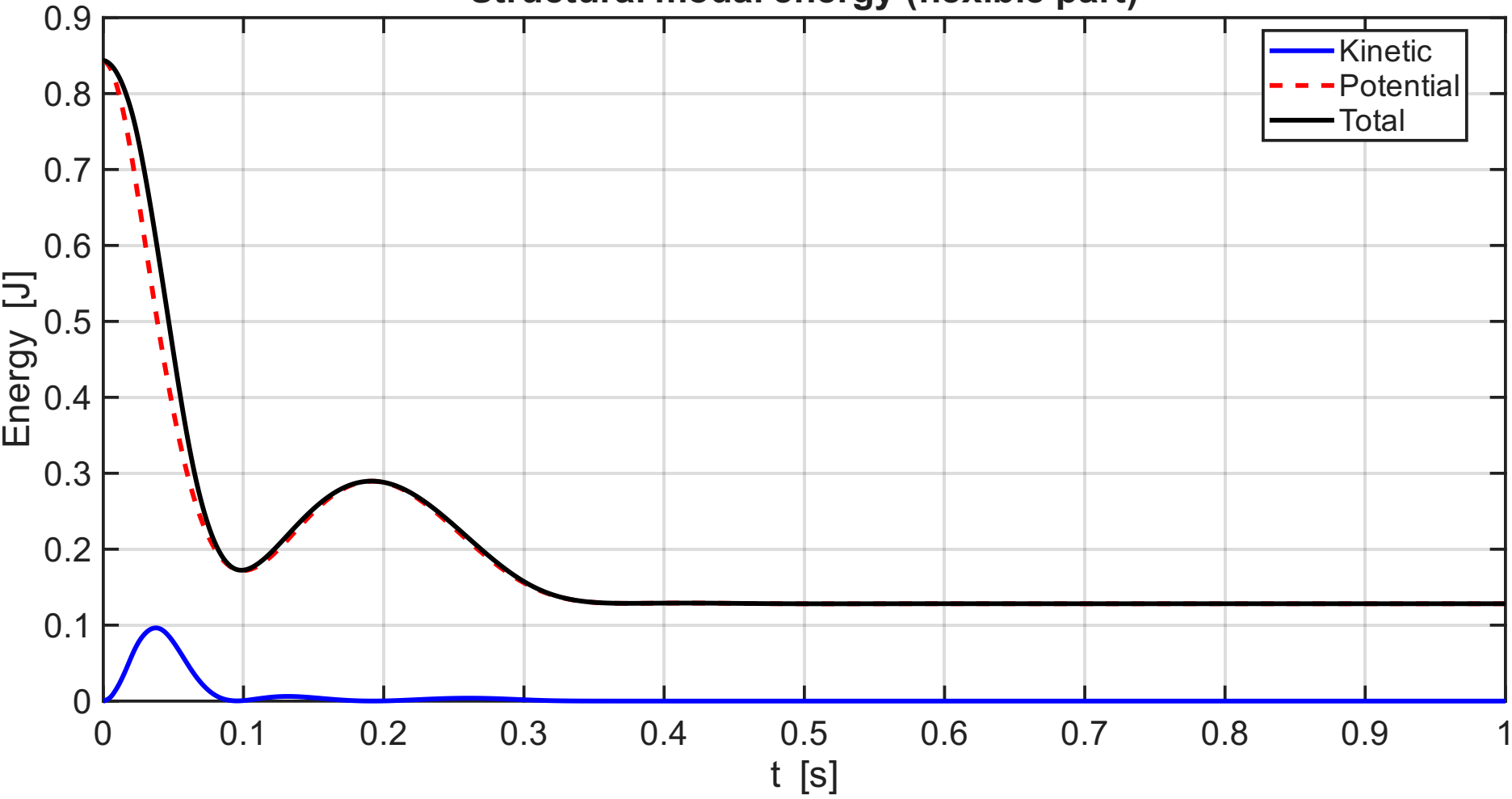
Structural modal energy (flexible part)
