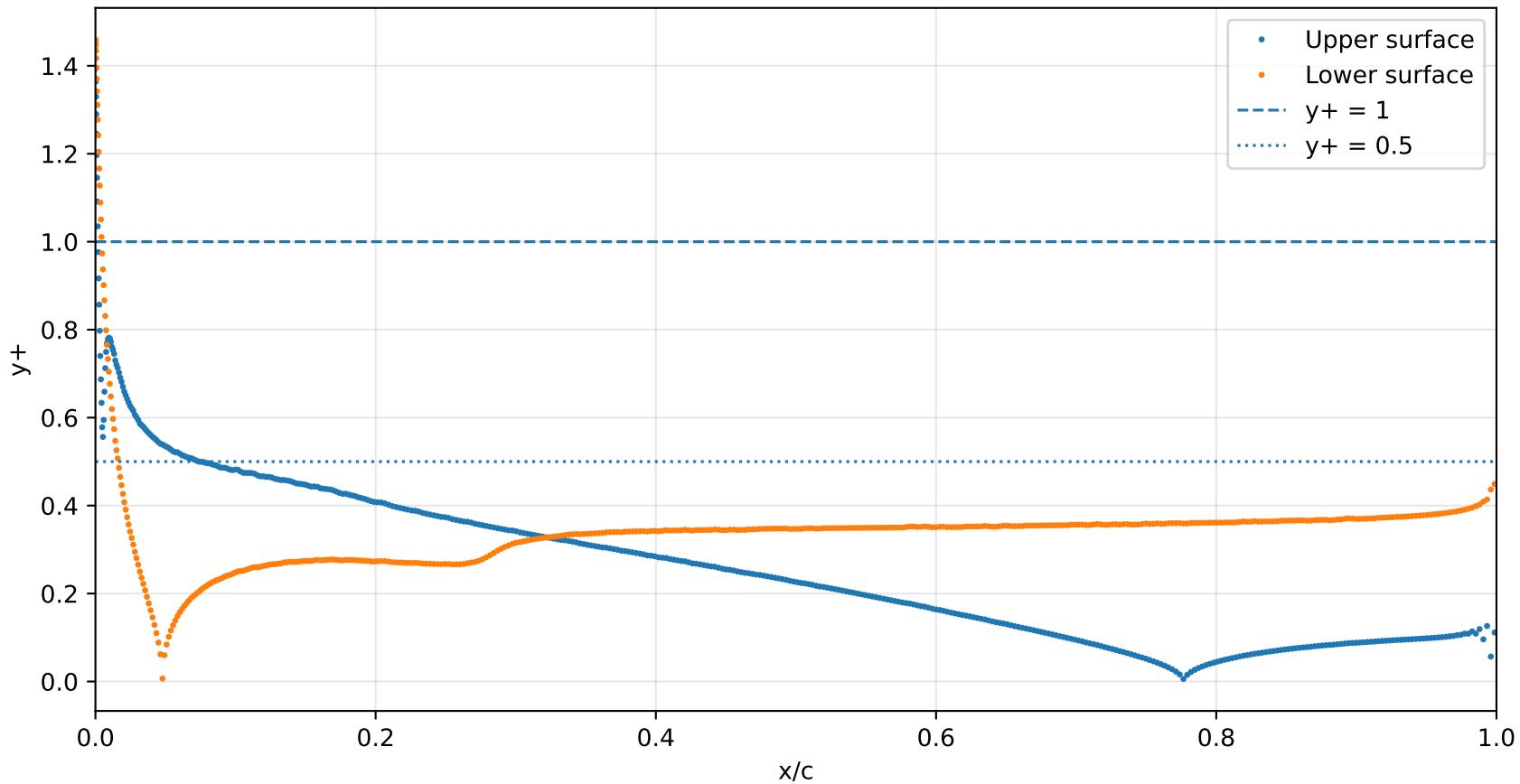
NACA0012 V9 — AoA 16° — Wall-adjacent y^+ distribution
