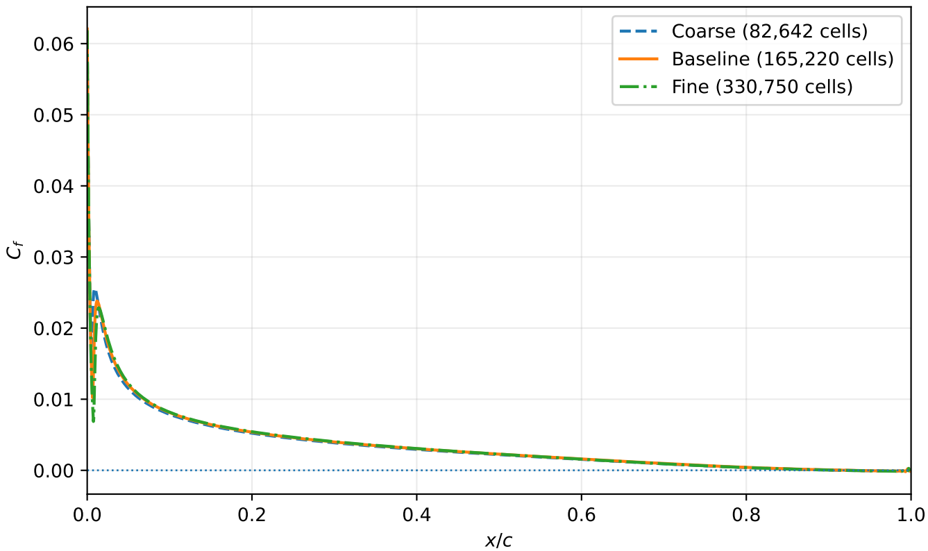
NACA 0012 upper-surface C_f , \alpha = 14^\circ
