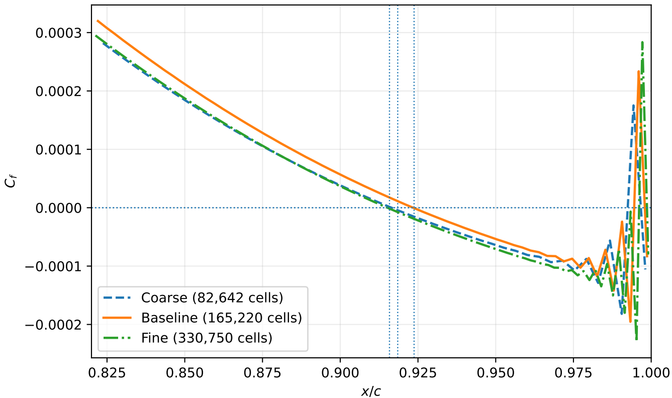
NACA 0012 upper-surface C_f : trailing-edge region, \alpha = 14^\circ
