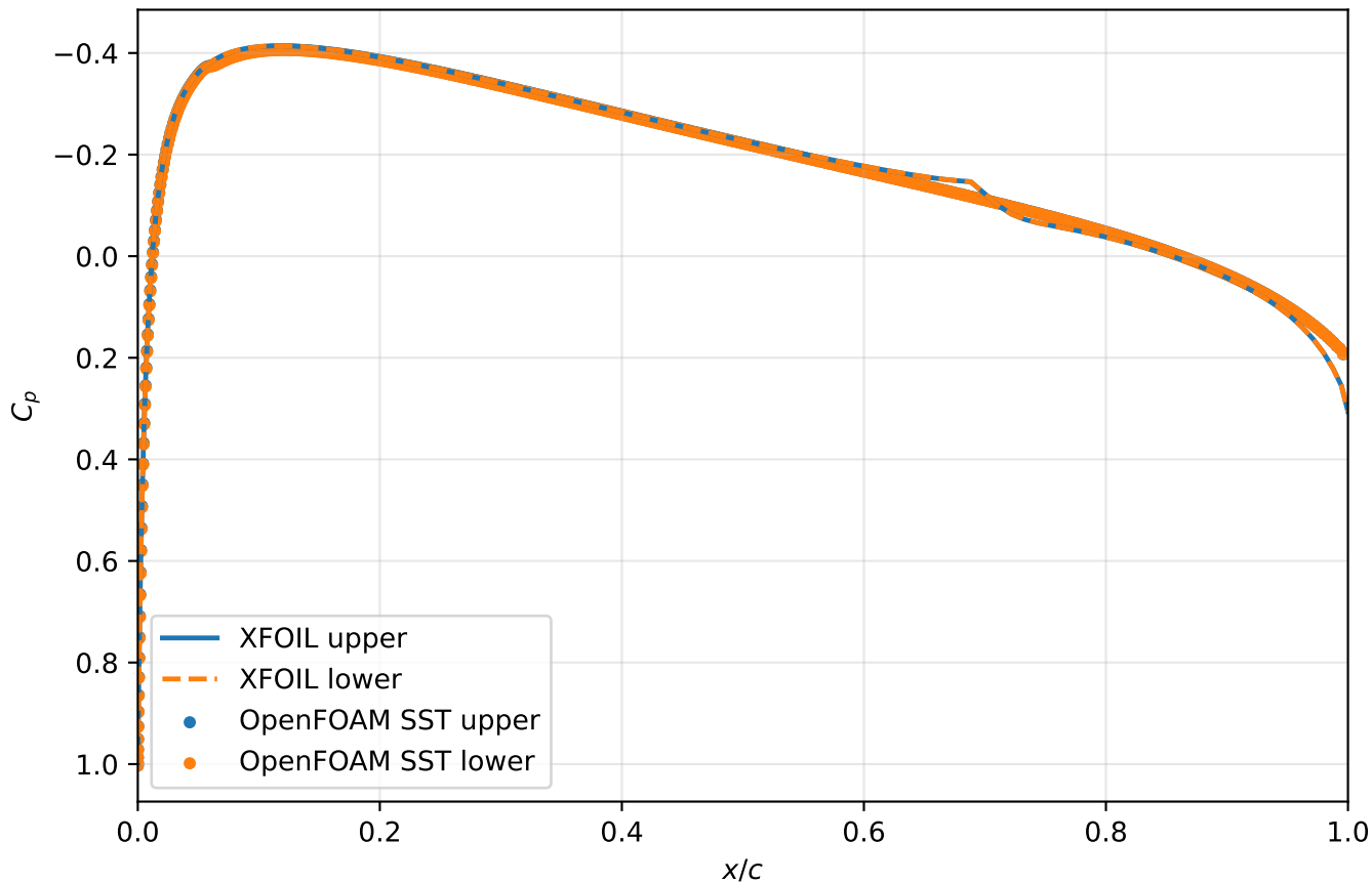
NACA0012, Re = 10^6 , AoA = 0^\circ
