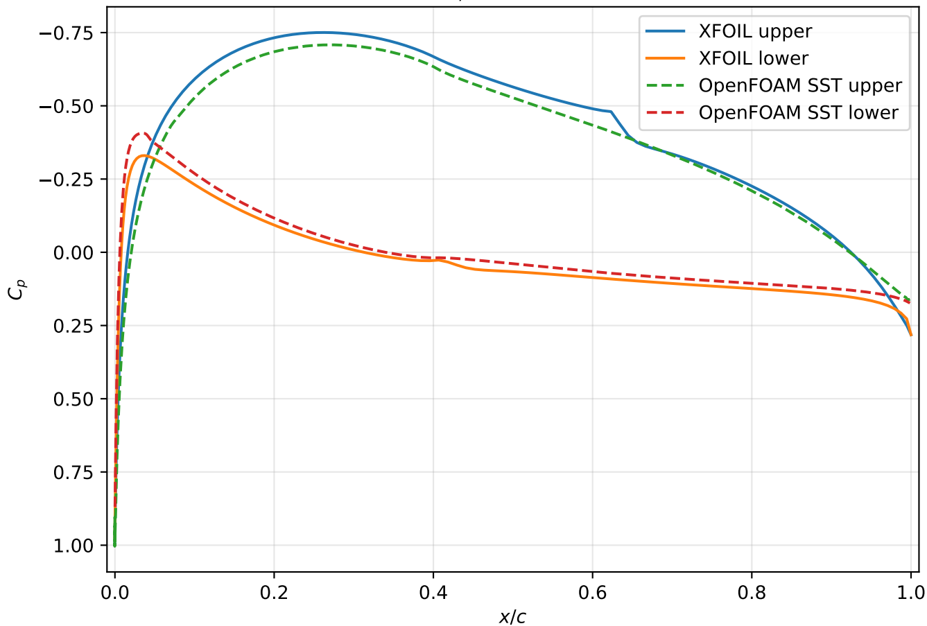
NACA4412: C_p comparison, \alpha = 0.0^\circ
