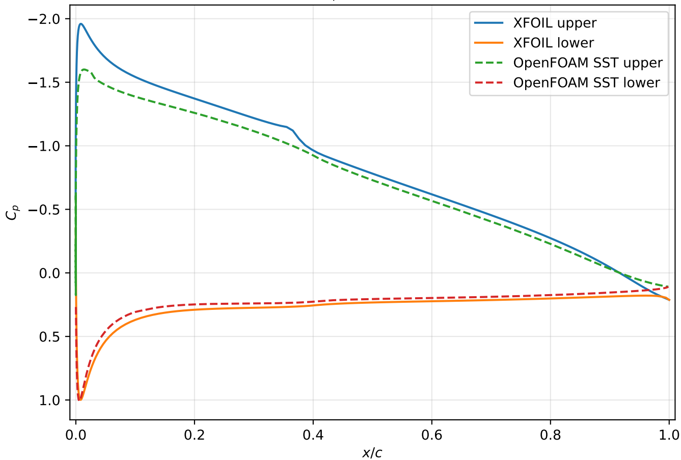
NACA4412: C_p comparison, \alpha = 6.0^\circ
