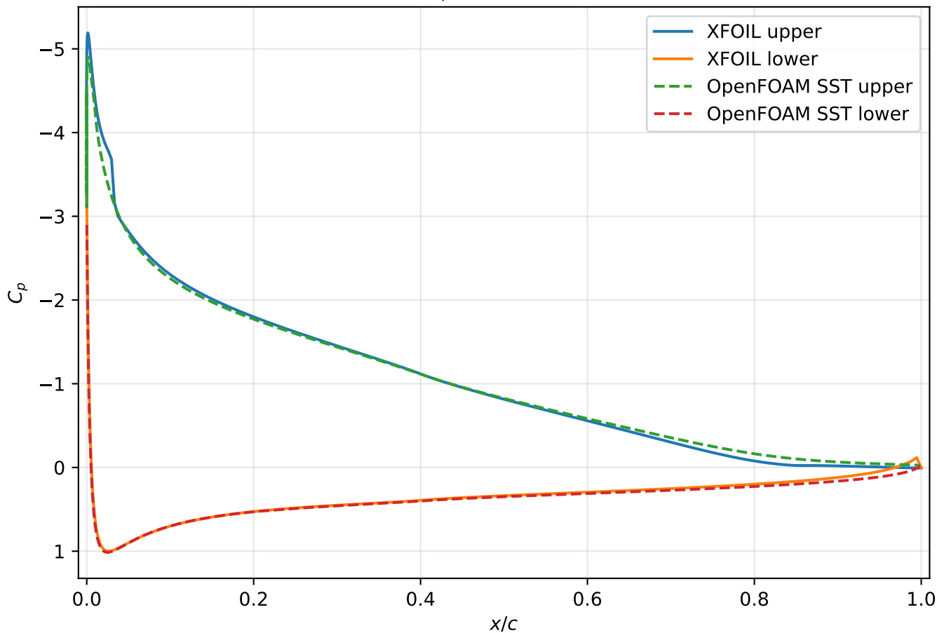
NACA4412: C_p comparison, \alpha = 12.0^\circ
