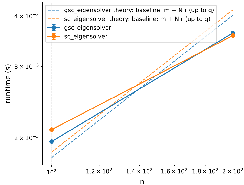
Eigensolver Network
