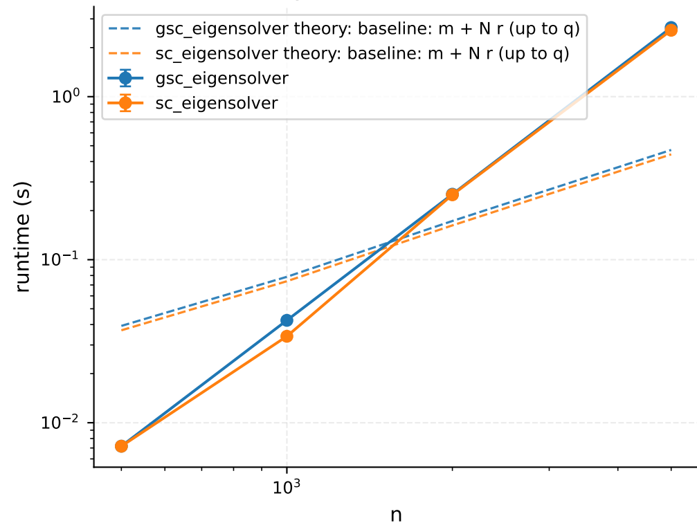
Eigsolver Pointcloud
