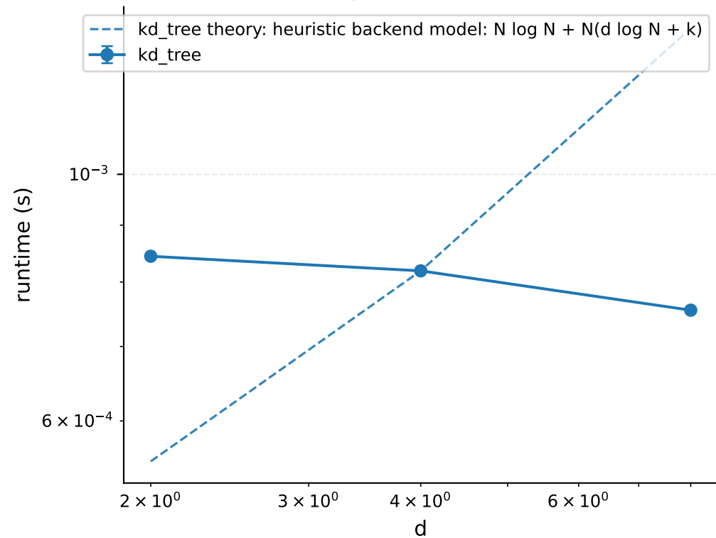
Graph Construction
