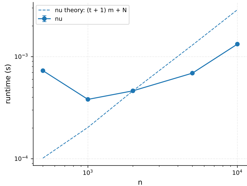
Measure Construction
