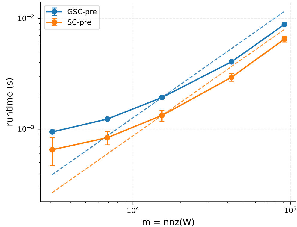
SC vs GSC preprocessing
