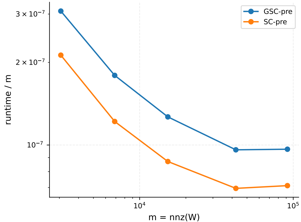
Deviation from linear sparse scaling
