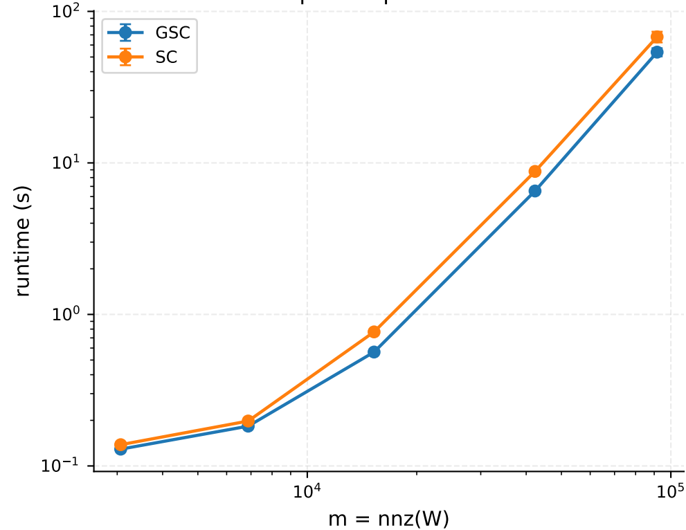
SC vs GSC on precomputed DISBM networks
