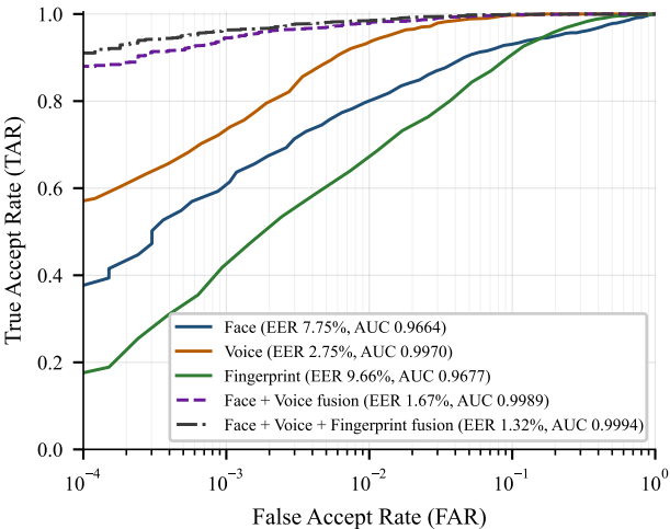
ROC, 256-bit protected templates (1,440 genuine / 33,120 impostor attempts)
