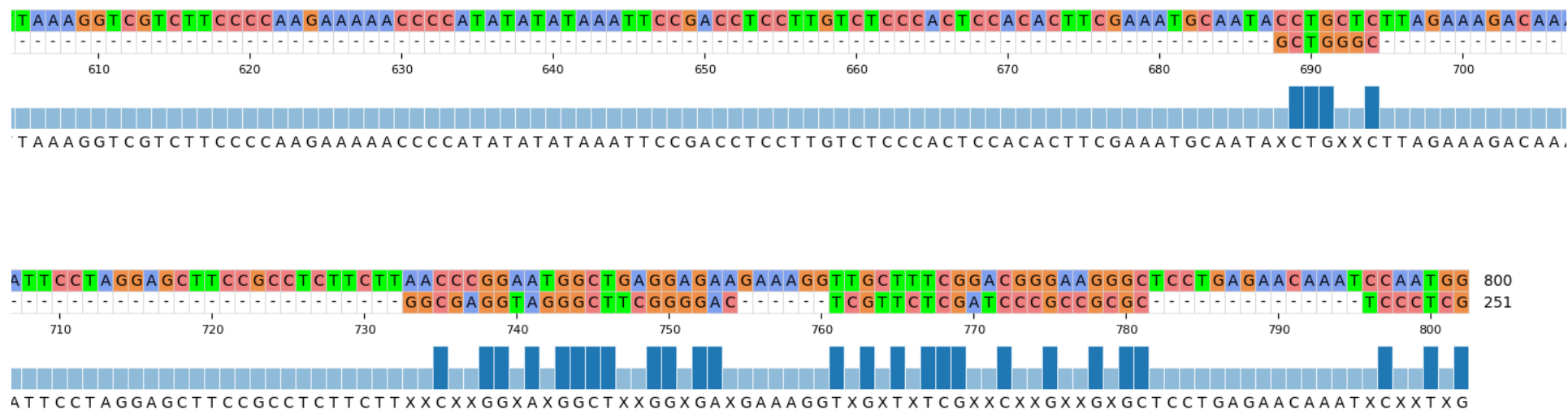
Figure 1. MSA - ITS2.fasta.
