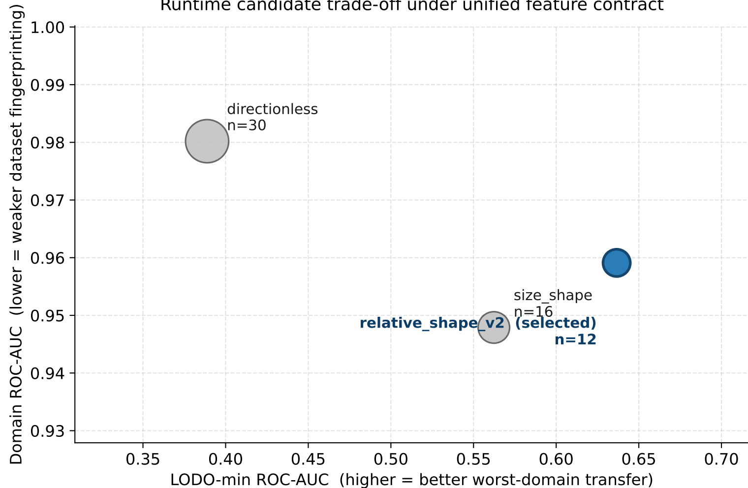
Runtime candidate trade-off under unified feature contract
