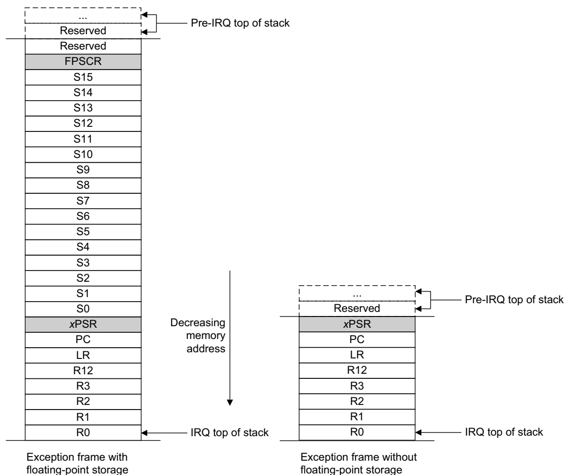
Figure 2-2 Exception stack frame
