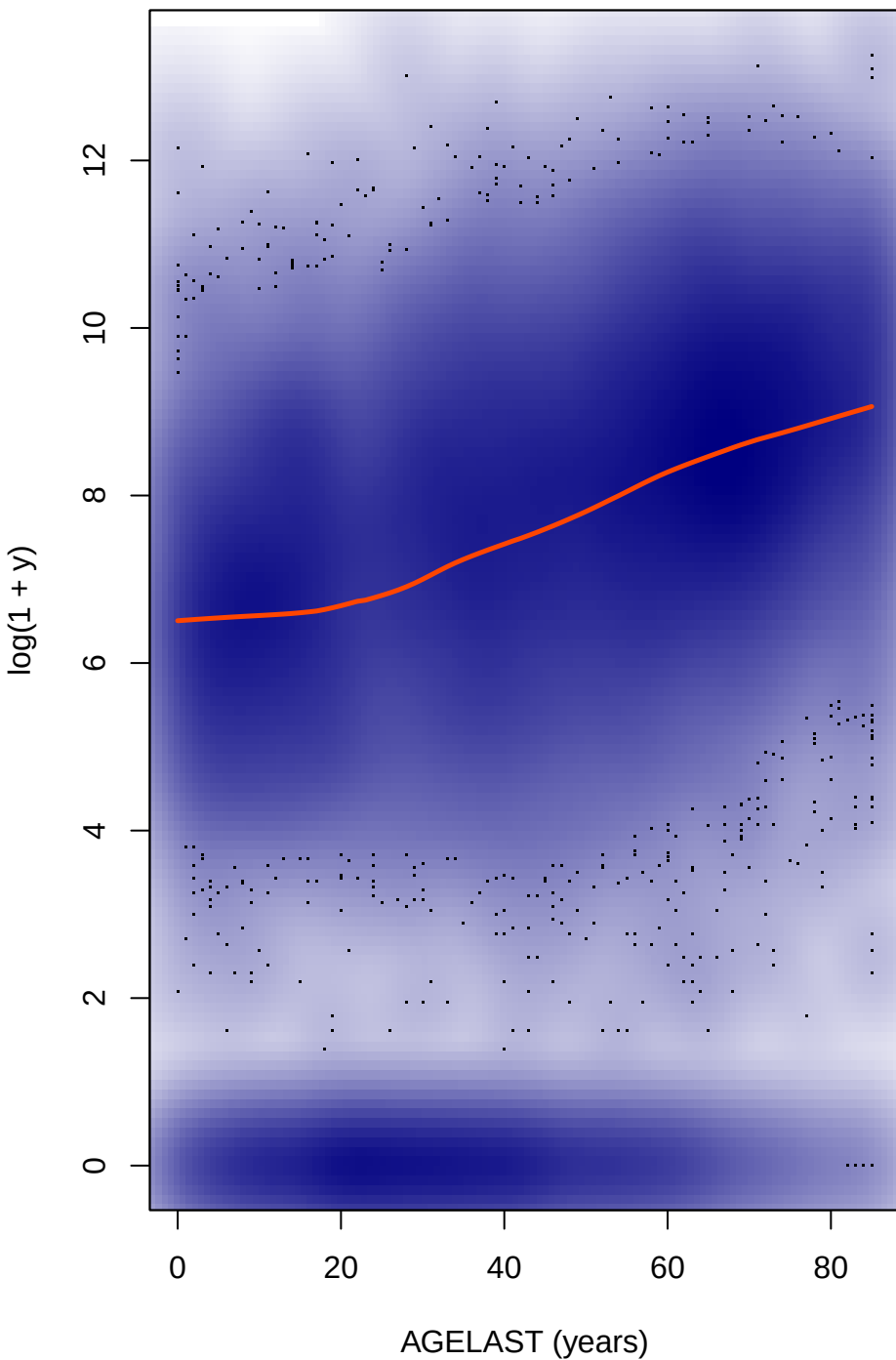
\log(1 + y) vs age (density)
