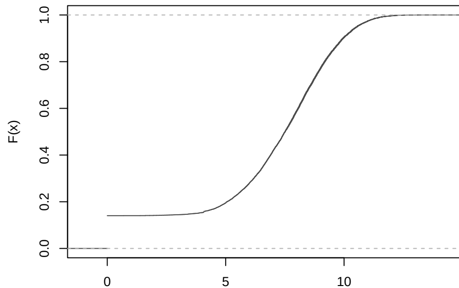
ECDF of log(1 + y)
