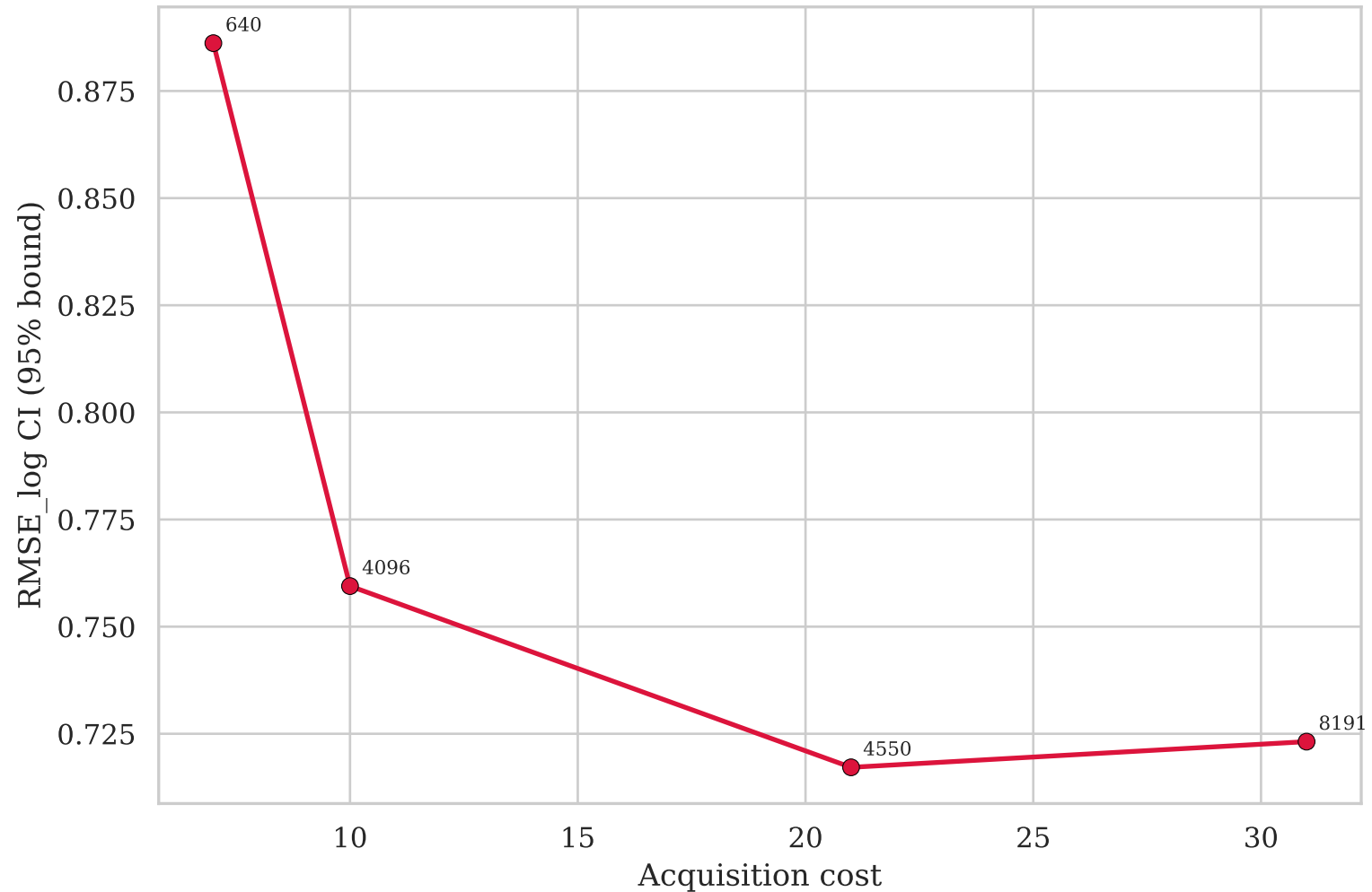
Nested LOWO: Cost vs RMSE_log
