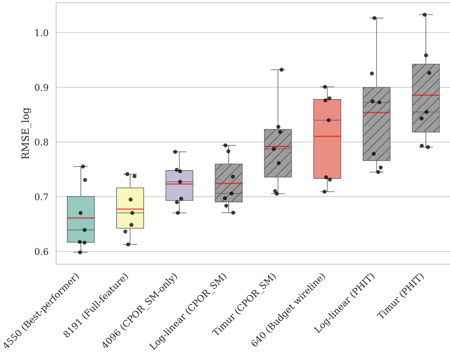
Nested LOWO per-well RMSE_log: subsets vs petrophysical baselines Sorted by mean, best at left; red line = mean
