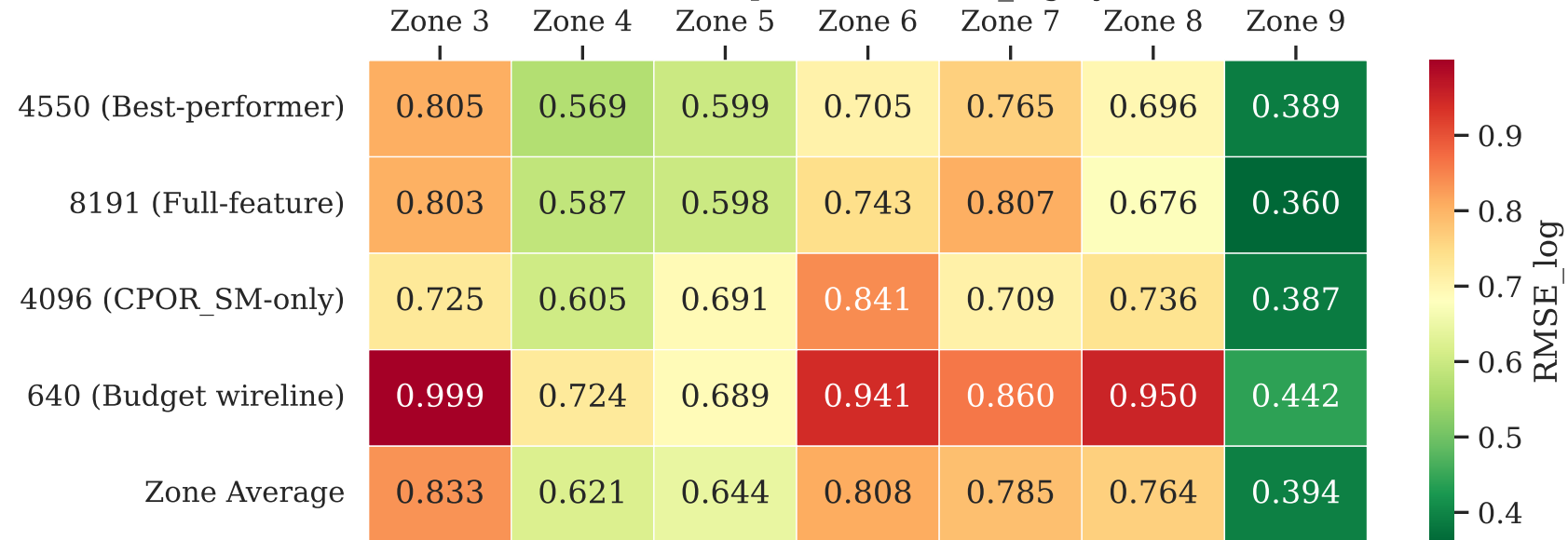
Nested LOWO per-zone RMSE_log by subset
