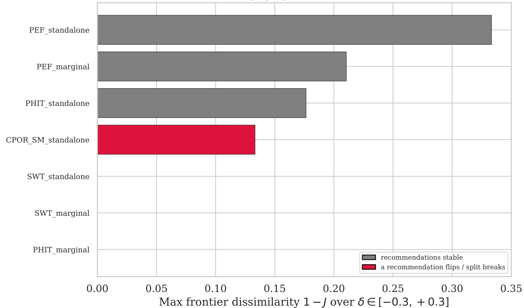
OAT cost sensitivity (gray = all recommendations stable)
