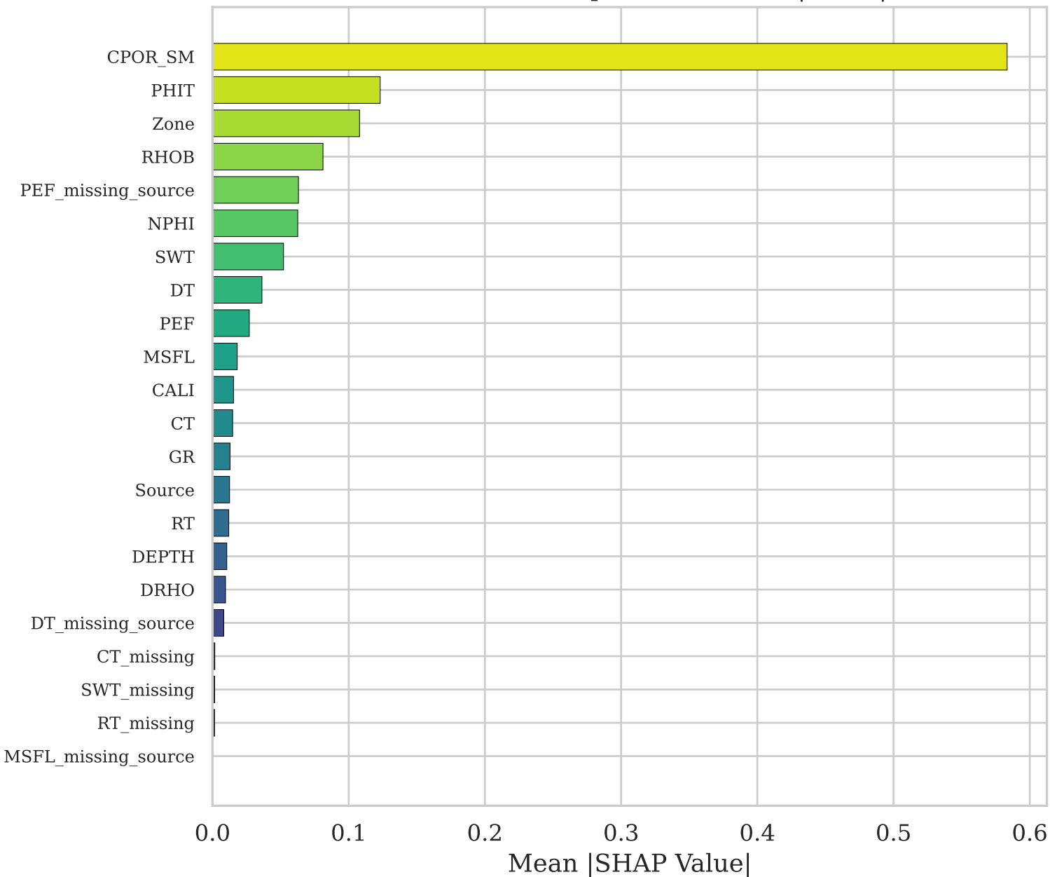
Global Feature Importance (Mean |SHAP|)
