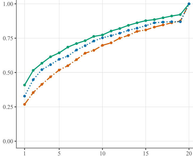
BugNet Python
