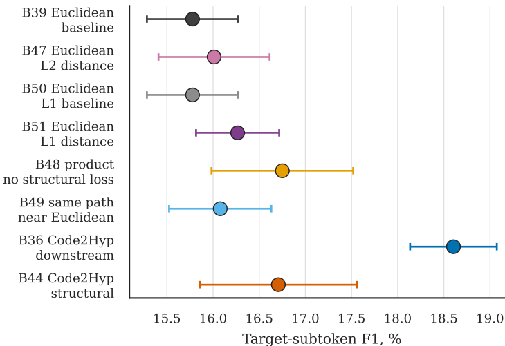
C. Metric distortion
