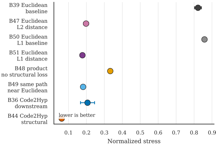
C. Metric distortion
