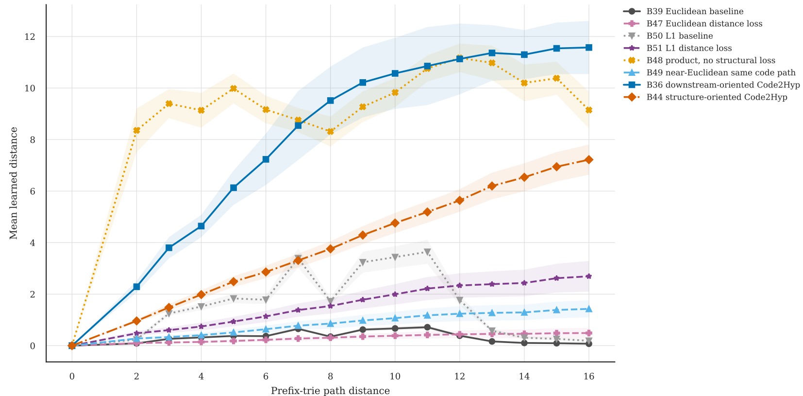
Learned structural distance by prefix-trie target level
