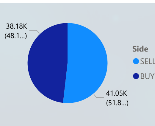
Buy vs Sell Distribution
