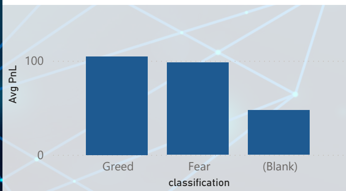
Avg PnL by Sentiment
