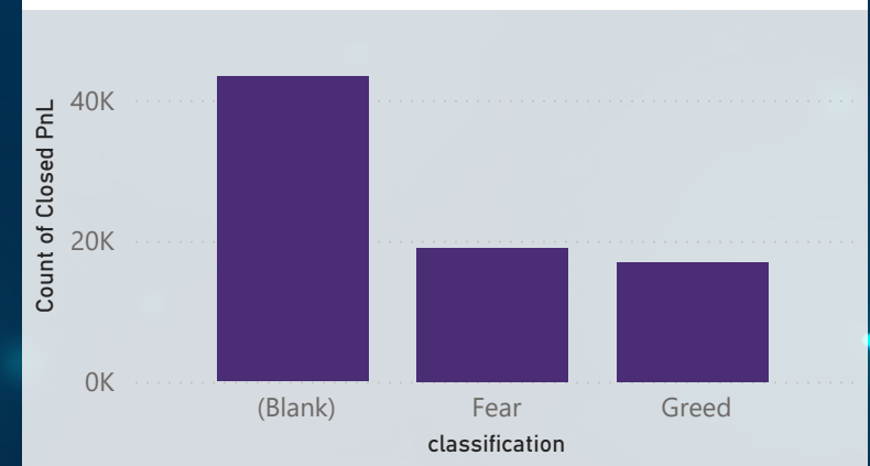
Count of Closed PnL by classification
