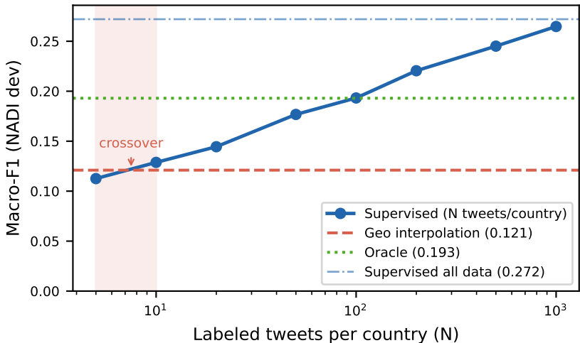
Annotation cost vs. ~zero-shot geographic interpolation
