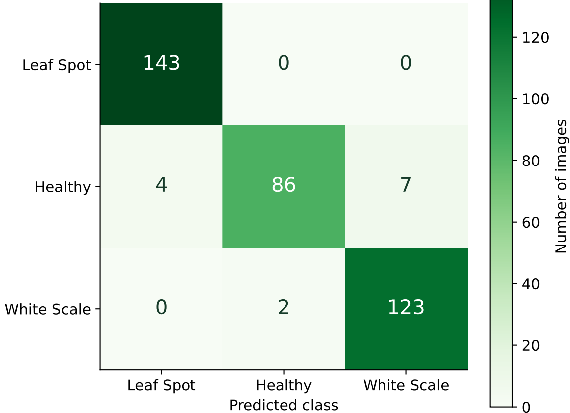
Confusion Matrix — New Test Set (n=365)
