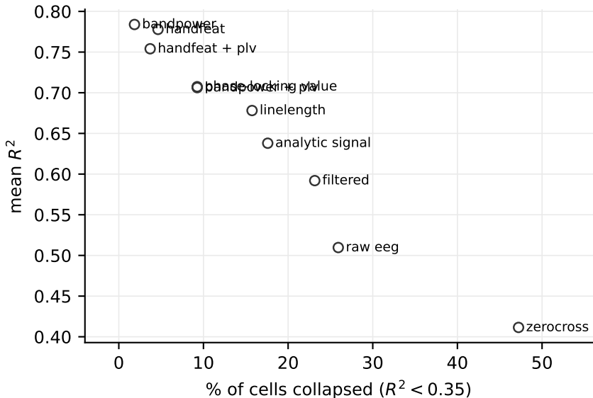
Feature ranking tracks collapse rate ( r = -0.98 )
