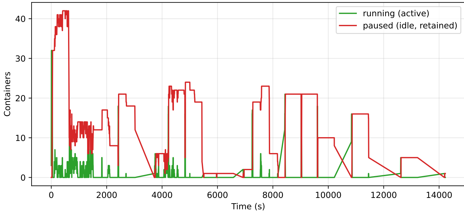
Running vs paused containers over time
