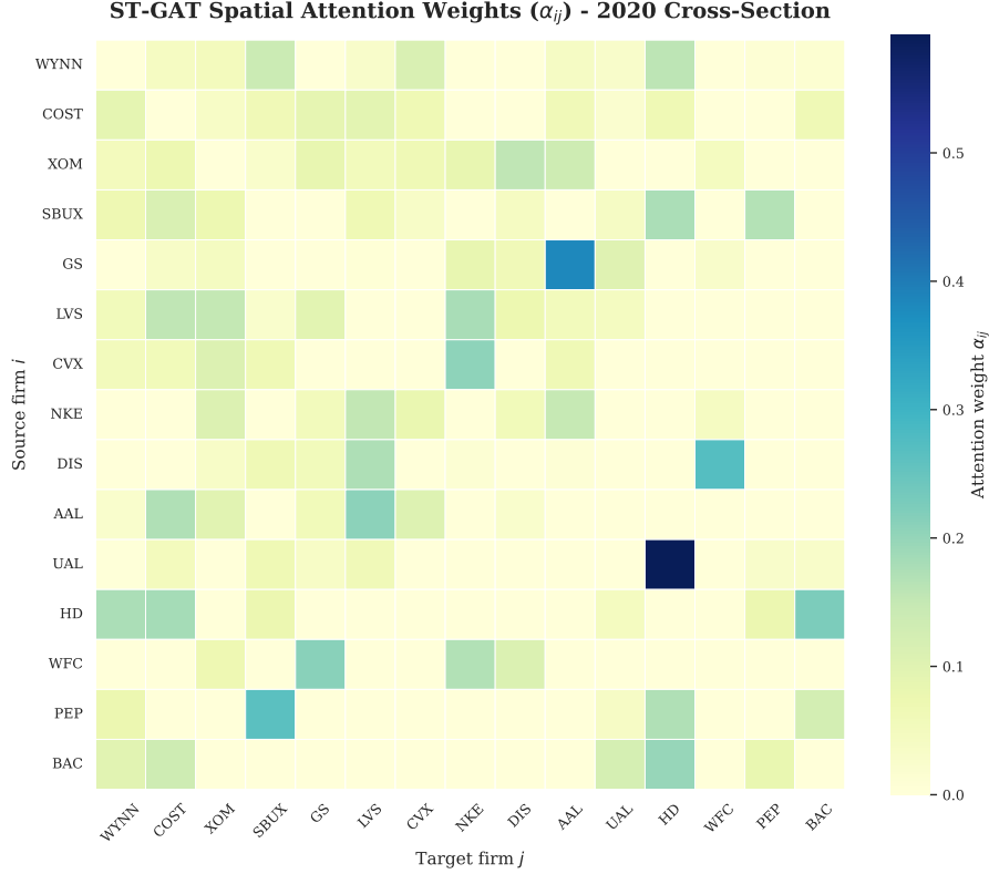
Figure 14: ST-GAT Spatial Attention Weights ( \alpha_{ij} ) for a subset of highly connected active nodes during the 2020 COVID-19 shock. The heatmap empirically demonstrates the network’s ability to dynamically route information across firms with high semantic risk similarity, validating the attention mechanism’s departure from a uniform or static industry-classification topology.
