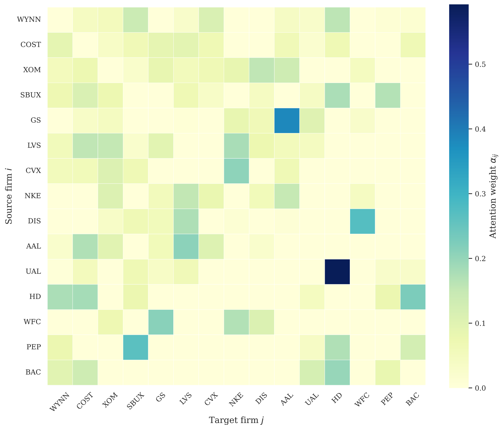
ST-GAT Spatial Attention Weights ( \alpha_{ij} ) - 2020 Cross-Section
