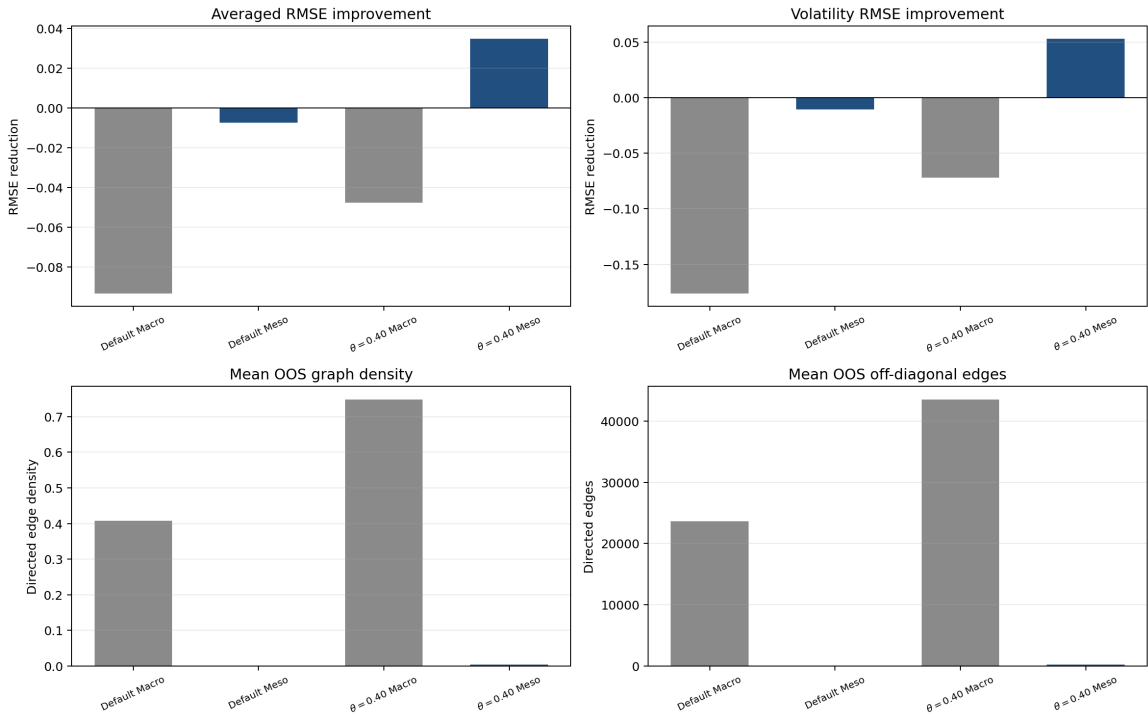
Figure 14: Downstream sensitivity dashboard for completed full-window taxonomy paths. Positive RMSE improvement indicates that ST-GAT outperforms its matched identity baseline. Graph density is averaged across 2021–2024 OOS years.
