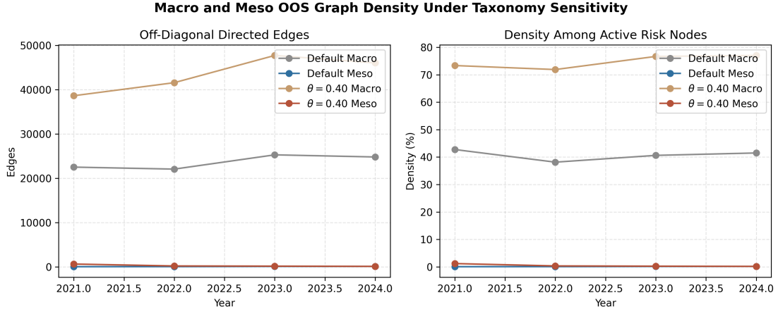
Figure 13: Empirical graph-density comparison for the OOS years, generated from the paired Macro and Meso graph-diagnostics CSV files under the default and \theta = 0.40 taxonomy paths.
