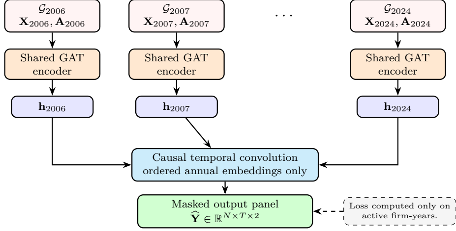
Figure 10: Temporal processing of annual graph snapshots. The shared GAT encoder is applied to each annual graph, and a causal temporal convolution produces masked return-volatility predictions across the full panel.
