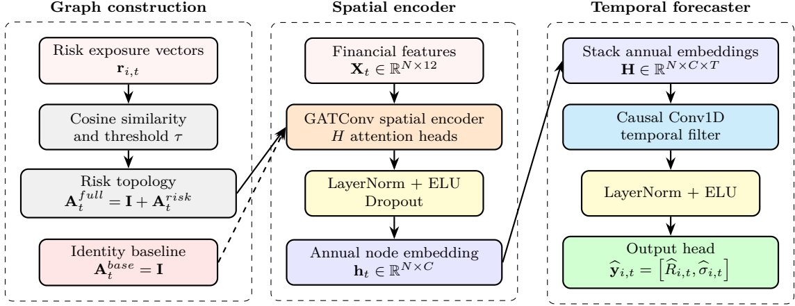
Figure 9: ST-GAT block architecture and identity-matrix ablation. Risk exposure vectors define the sparse graph topology, financial node features enter the spatial GAT encoder, and annual embeddings are passed through a causal temporal forecaster to predict one-year-ahead return and volatility. The full model uses textual peer topology, whereas the identity baseline removes all off-diagonal links. Cosine similarity determines edge existence, while attention weights are learned by GATConv.
