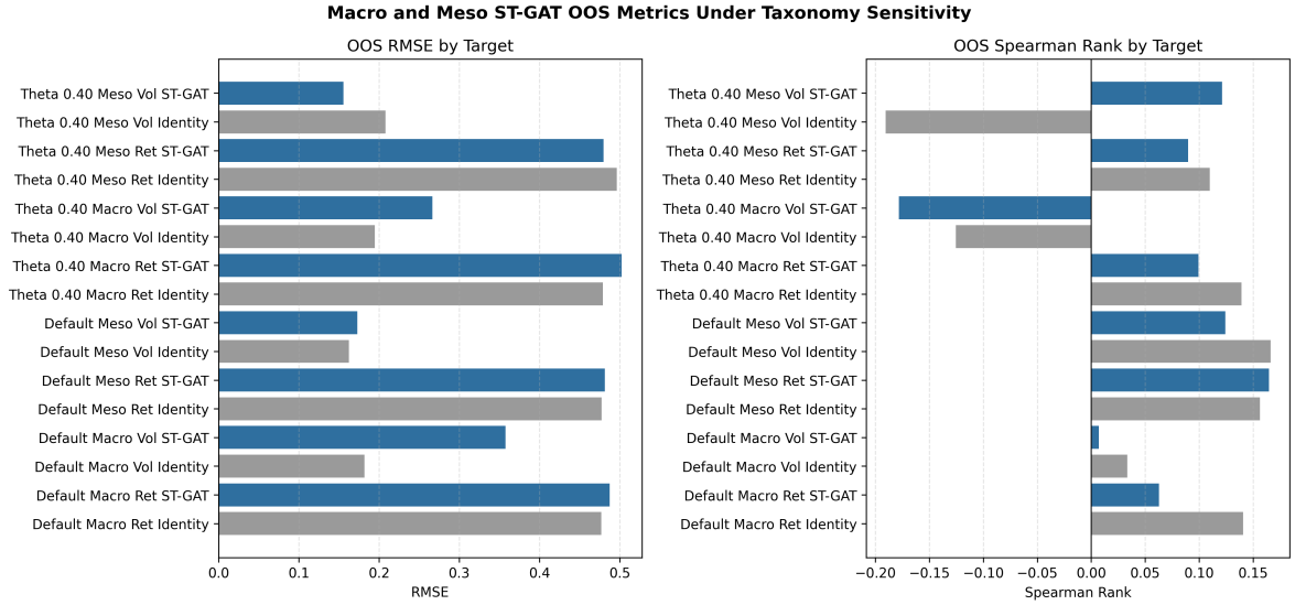
Figure 11: Empirical OOS metric comparison for Macro and Meso ST-GAT specifications under the default and \theta = 0.40 taxonomy paths. Lower RMSE is better; higher Spearman rank correlation is better.
