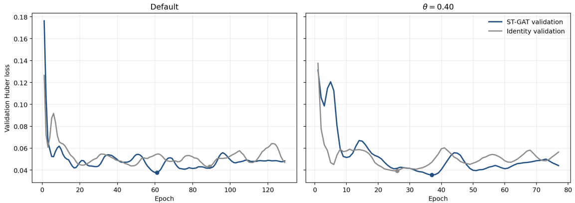
Figure 12: Validation Huber-loss convergence for ST-GAT and identity-baseline models under the default and \theta = 0.40 dynamic taxonomies. Dots mark the best validation checkpoints restored for OOS evaluation.
