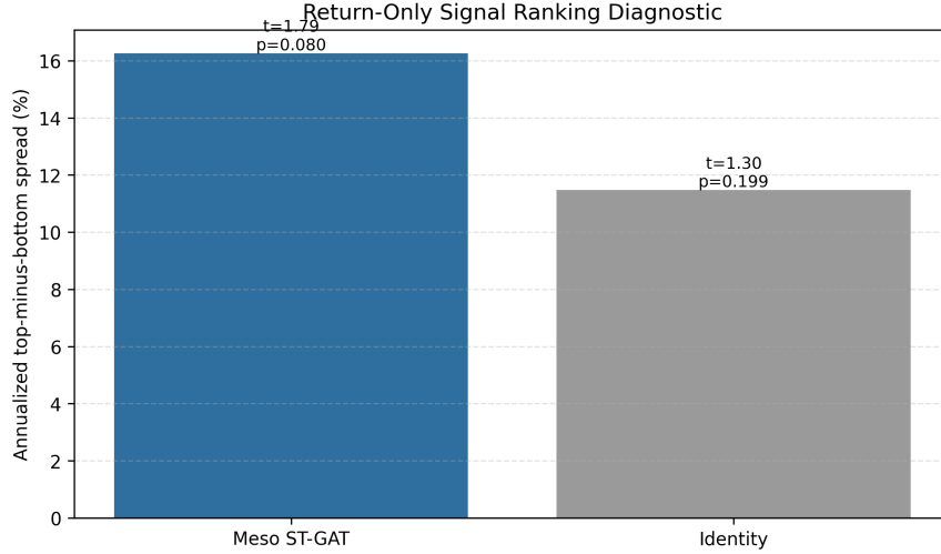
Figure 17: Return-only top-minus-bottom spread comparison for ST-GAT and identity-baseline signals. The reported p -values are nominal and not adjusted for multiple score/model comparisons.
