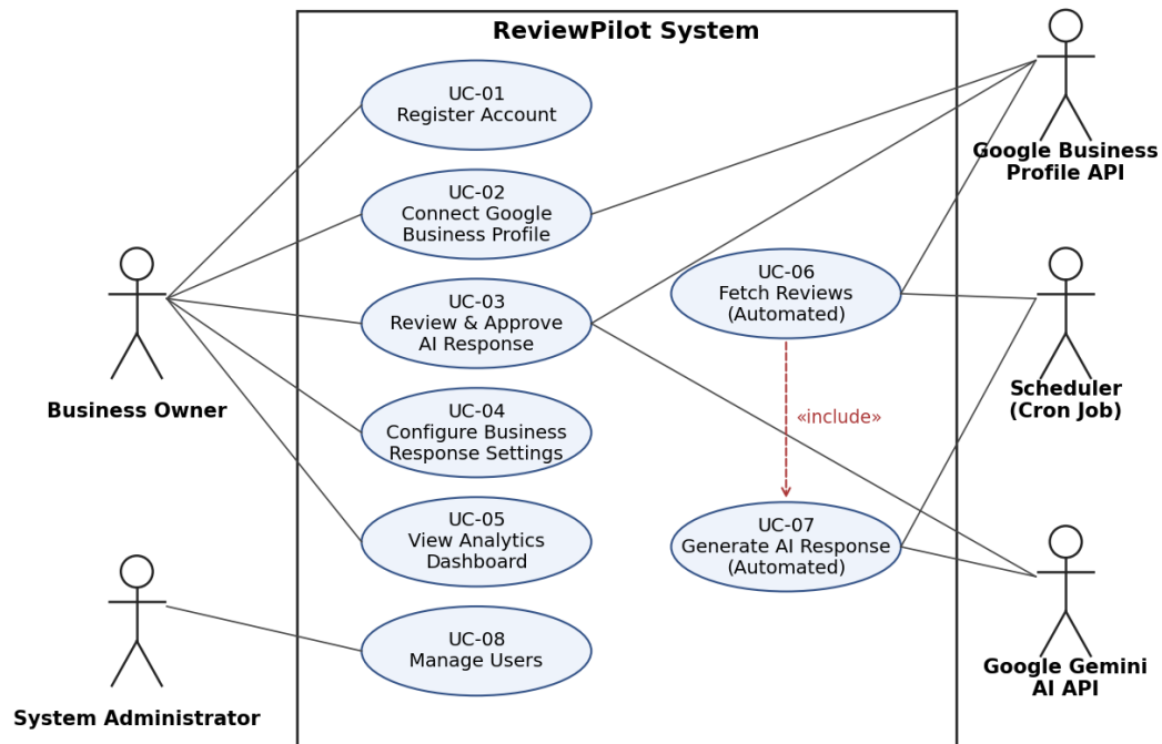
Figure 1 Use case diagram of ReviewPilot
