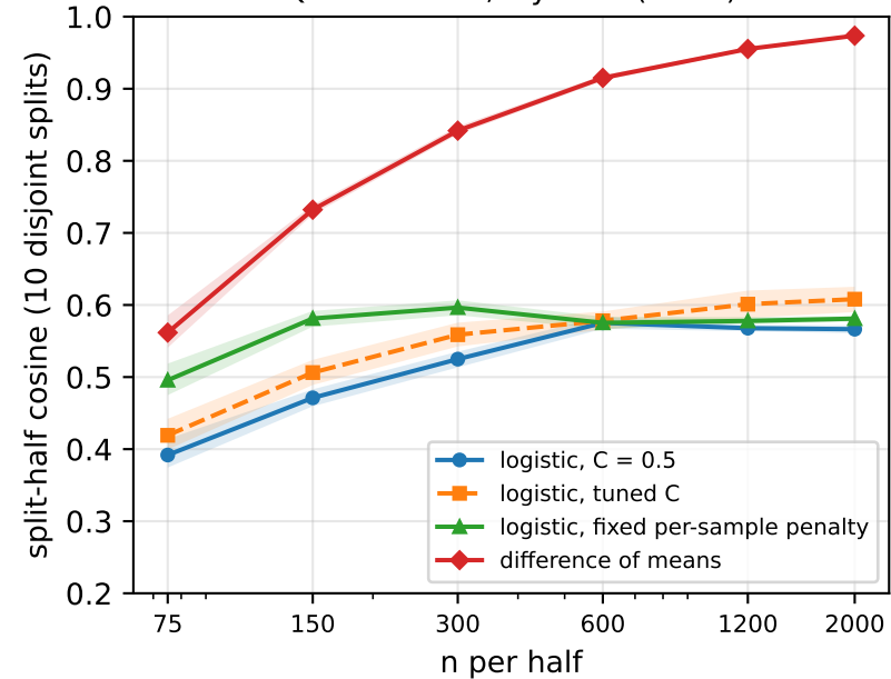
Qwen3.6-27B, layer 43 (focus)
