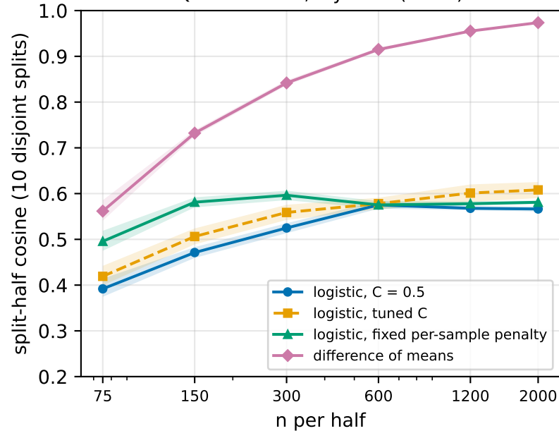
Qwen3.6-27B, layer 43 (focus)
