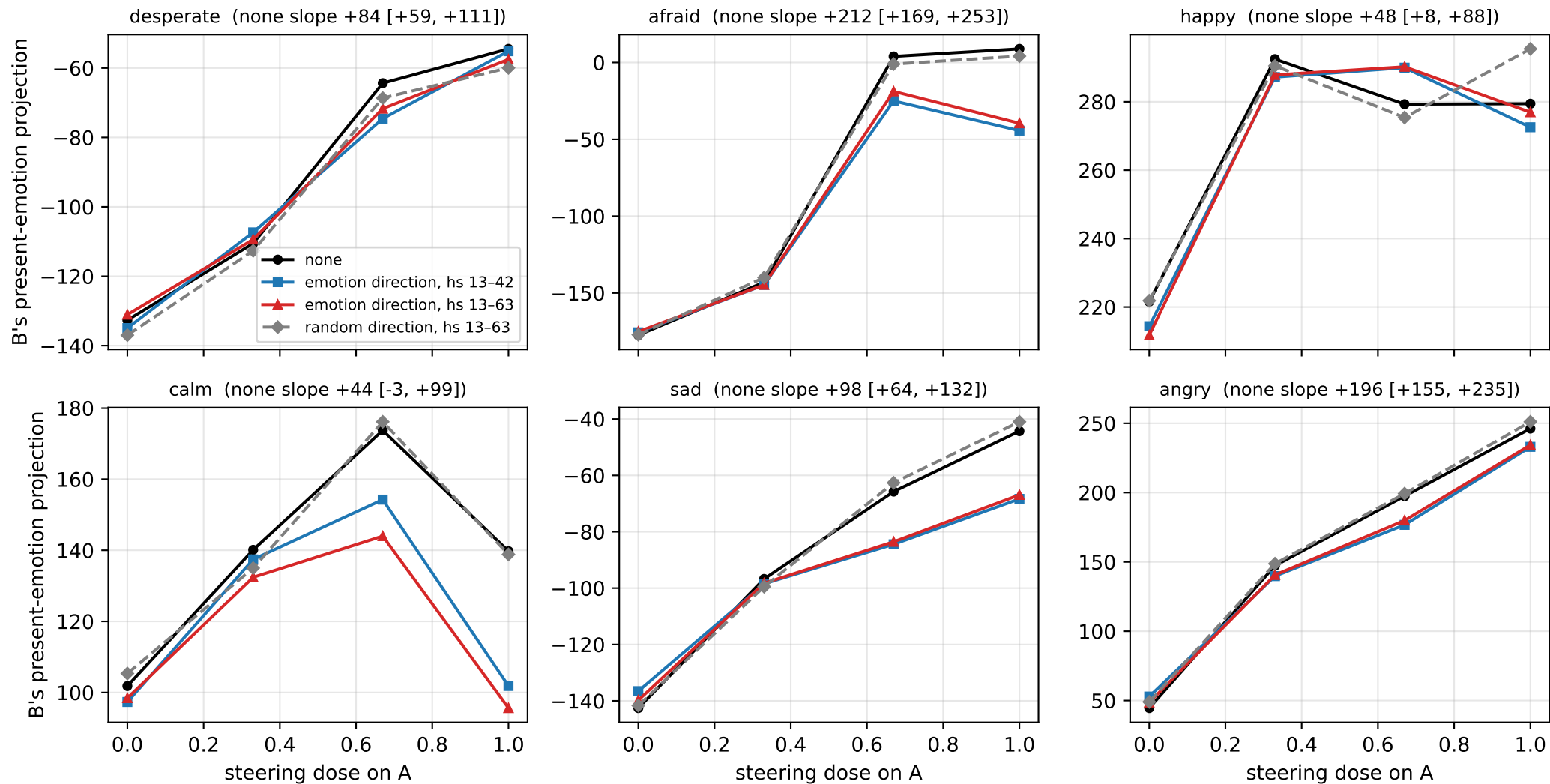
B1c: B's dose-response under all-layer ablation of A's span (29 scenarios \times 3 reps)
