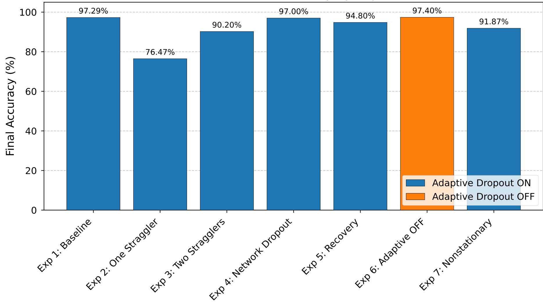
Final Global Model Accuracy by Experiment
