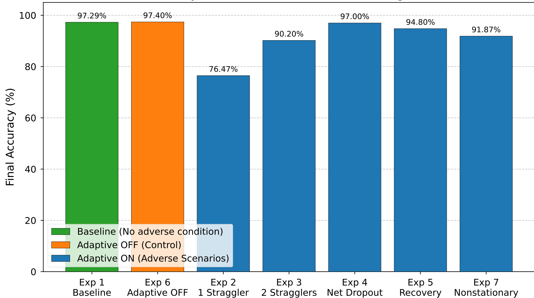
Final Accuracy Under Tested Federated Learning Scenarios
