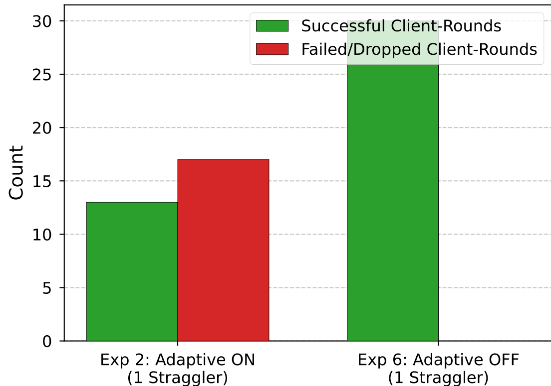
Client-Round Outcomes
