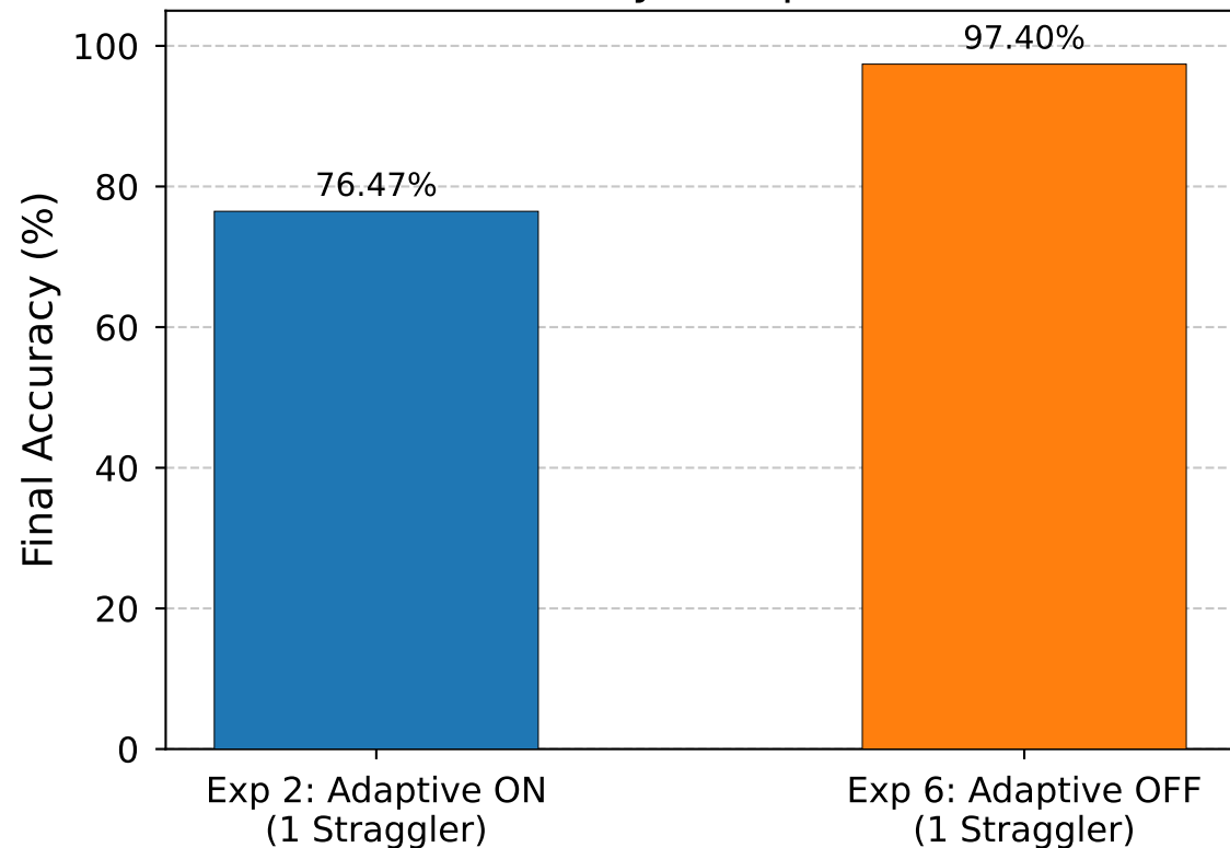
Accuracy Comparison
