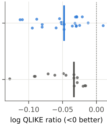
H4: kernel vs kNN analogue
