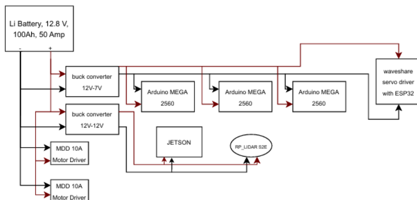
Figure 3.3: Power distribution diagram for battery, buck converters, and controllers.
