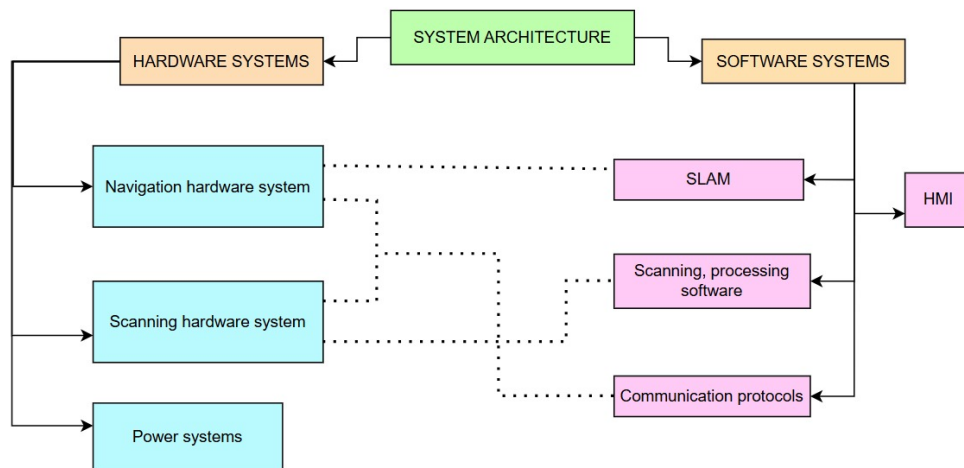
Figure 3.1: High level interaction between the rover's hardware subsystems and software stack.
