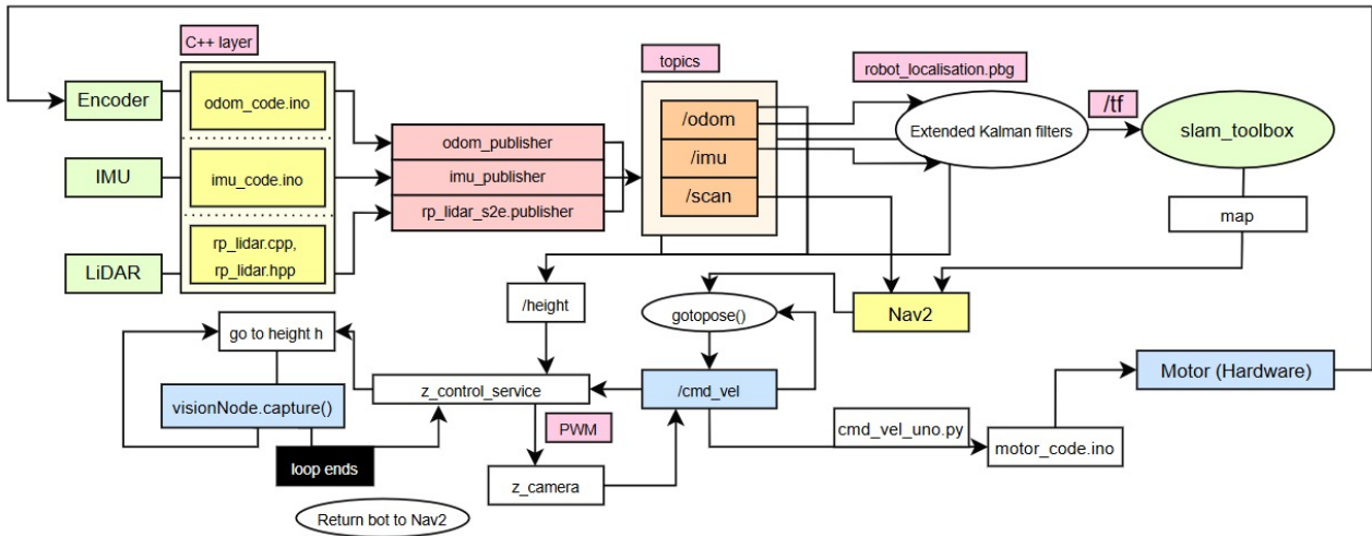
Figure 3.4: Software pipeline from sensors and vision node to SLAM, Nav2, and motor control.
