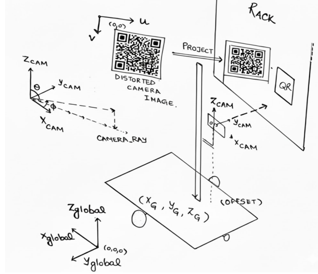
Figure 5.3: We use the above three coordinate frames to establish a 3D projection of image to a plane parallel to the rack (Geometric Rectification)
