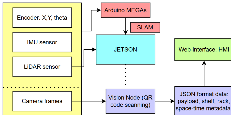
Figure 3.8: Block diagram of the Data flow from the sensors to the HMI
