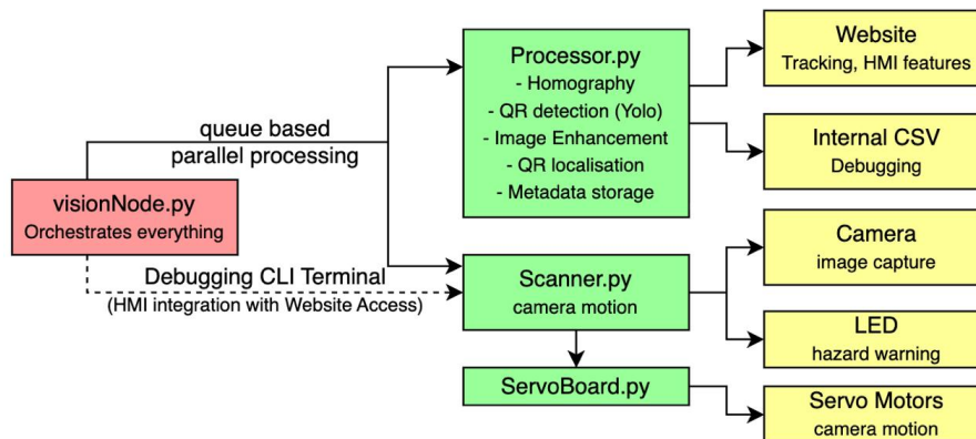
Figure 5.2: High level architecture of Vision Pipeline
