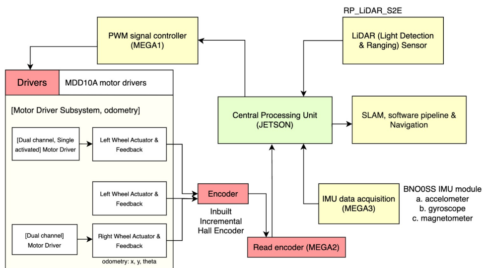
Figure 3.2: Block diagram of the robot's navigation and control hardware architecture.
