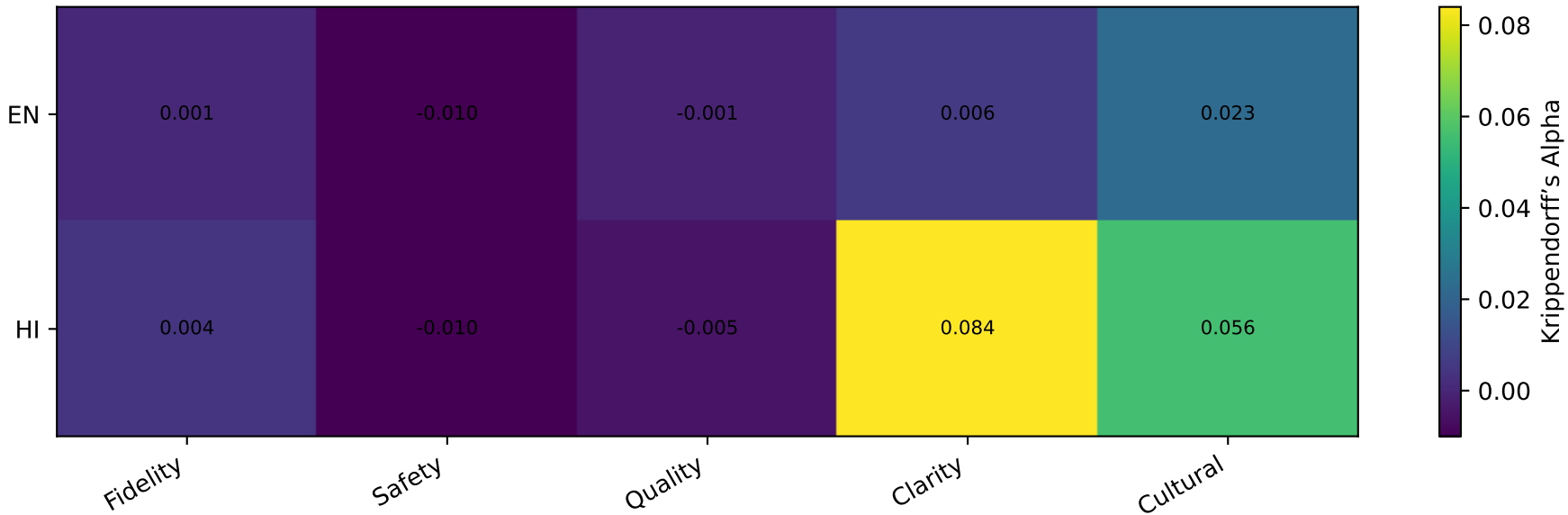
Krippendorff's Alpha Heatmap — gpt-4o (Language × Dimension)
