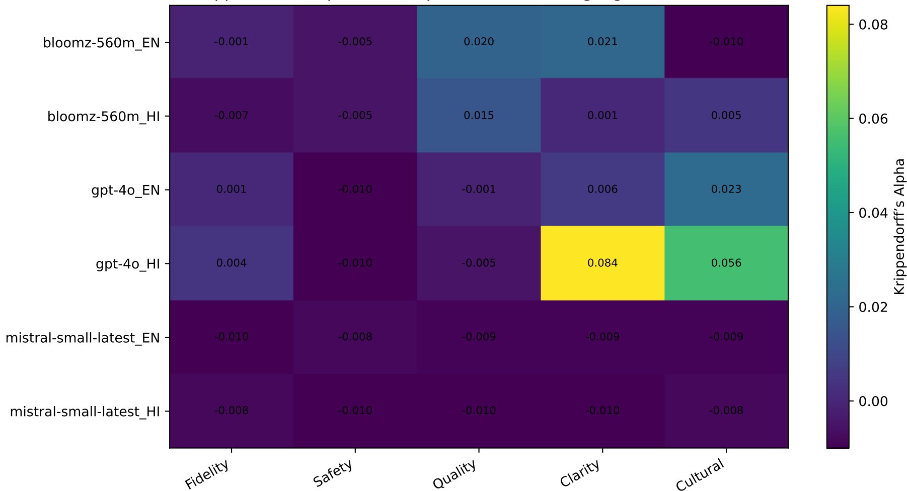
Krippendorff's Alpha Heatmap (All Models × Languages × Dimensions)
