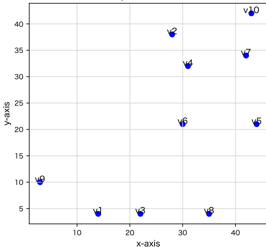
10 random points in a 50×50 Grid
