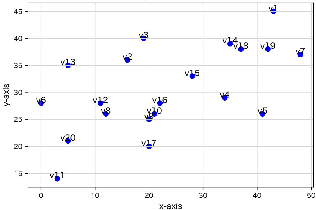
20 random points in a 50×50 Grid
