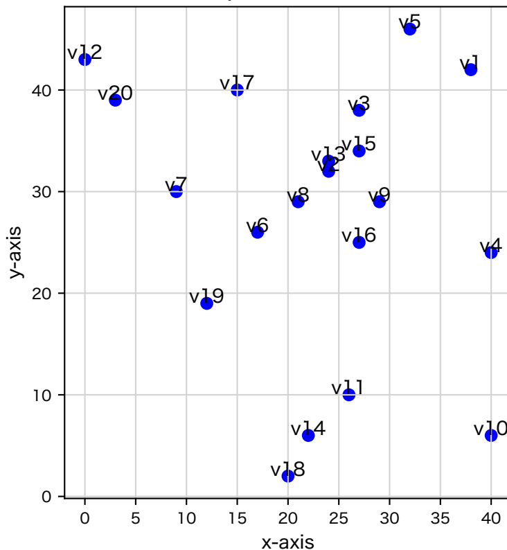
20 random points in a 50×50 Grid
