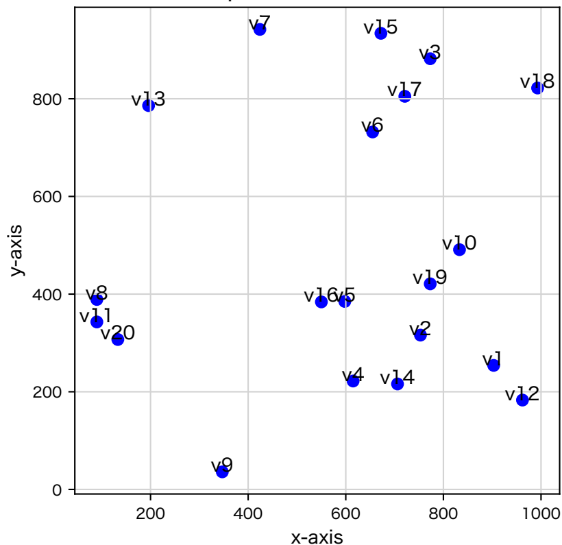
20 random points in a 1000×1000 Grid
