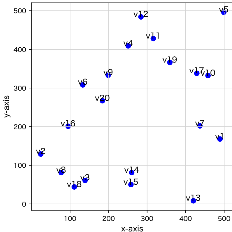
20 random points in a 500×500 Grid
