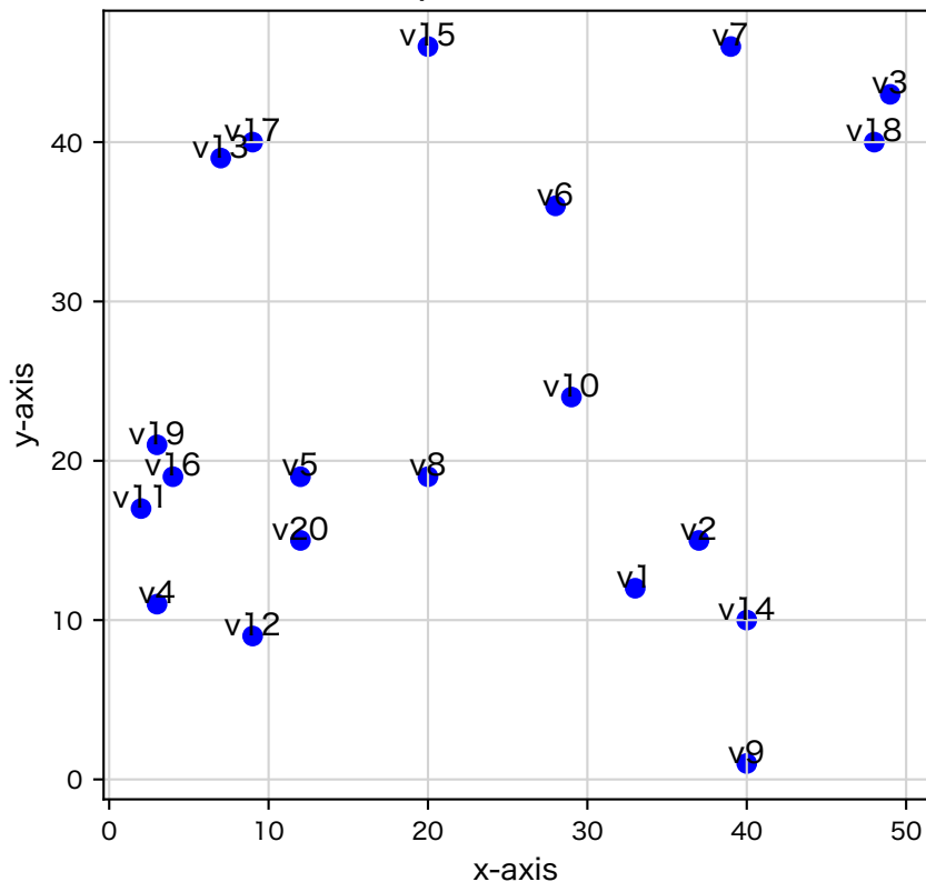
20 random points in a 50×50 Grid
