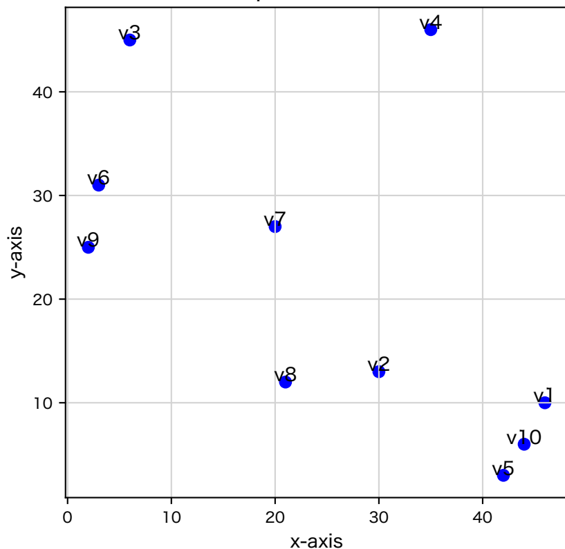
10 random points in a 50×50 Grid
