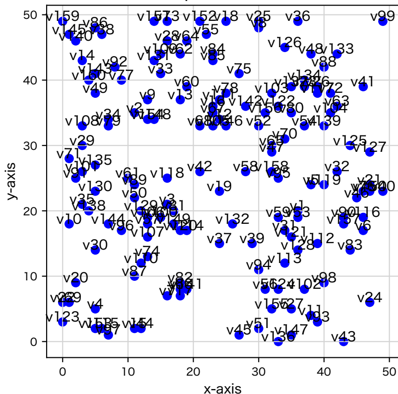
160 random points in a 50x50 Grid
