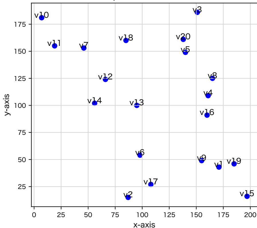
20 random points in a 200×200 Grid
