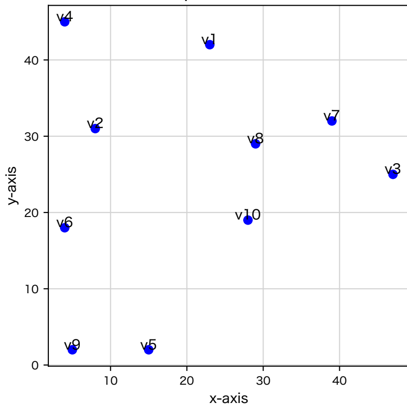
10 random points in a 50×50 Grid
