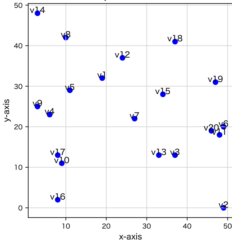
20 random points in a 50×50 Grid
