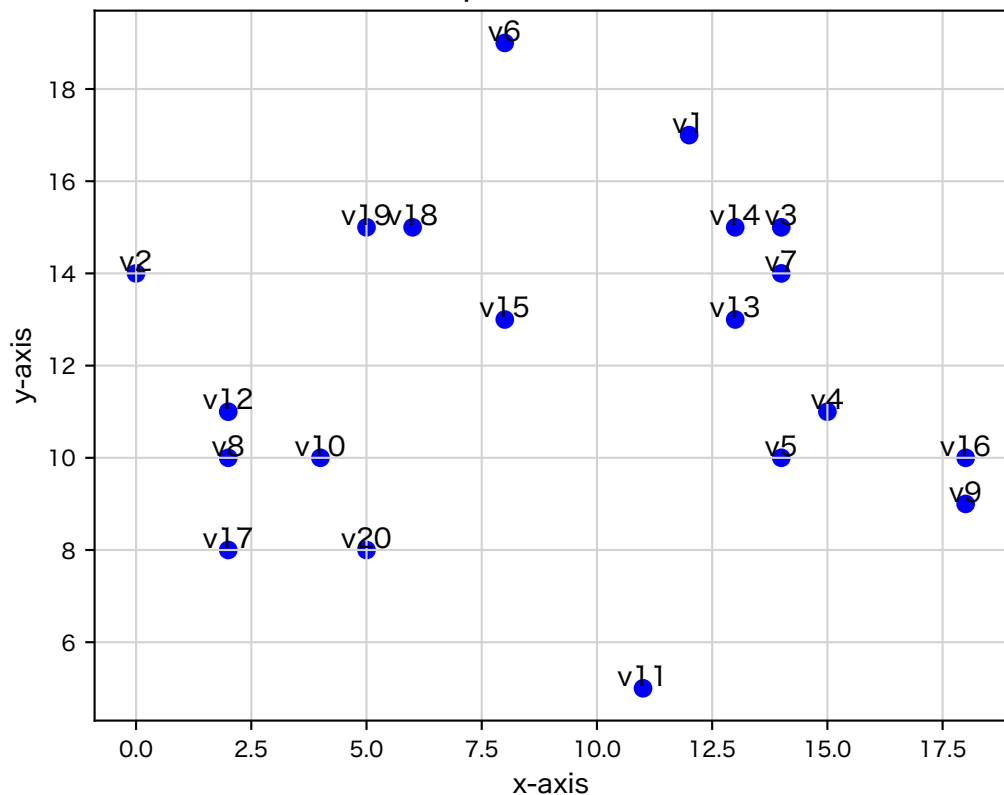
20 random points in a 20×20 Grid
