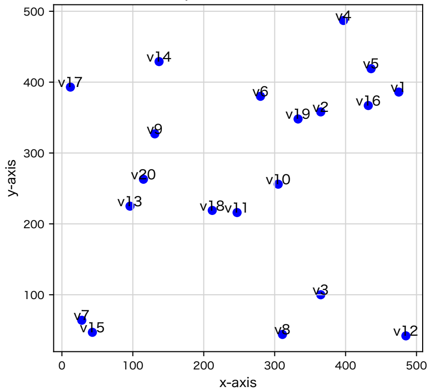
20 random points in a 500×500 Grid
