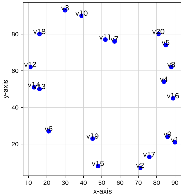
20 random points in a 100×100 Grid
