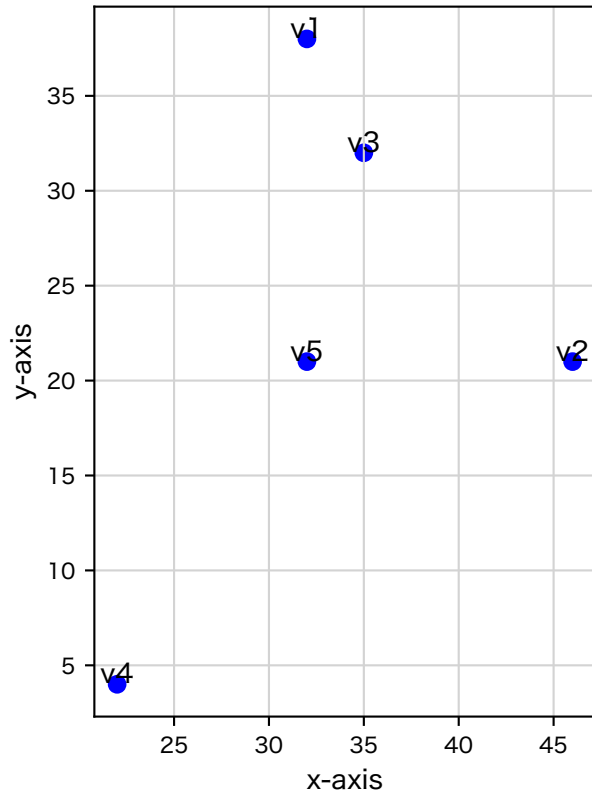
5 random points in a 50×50 Grid
