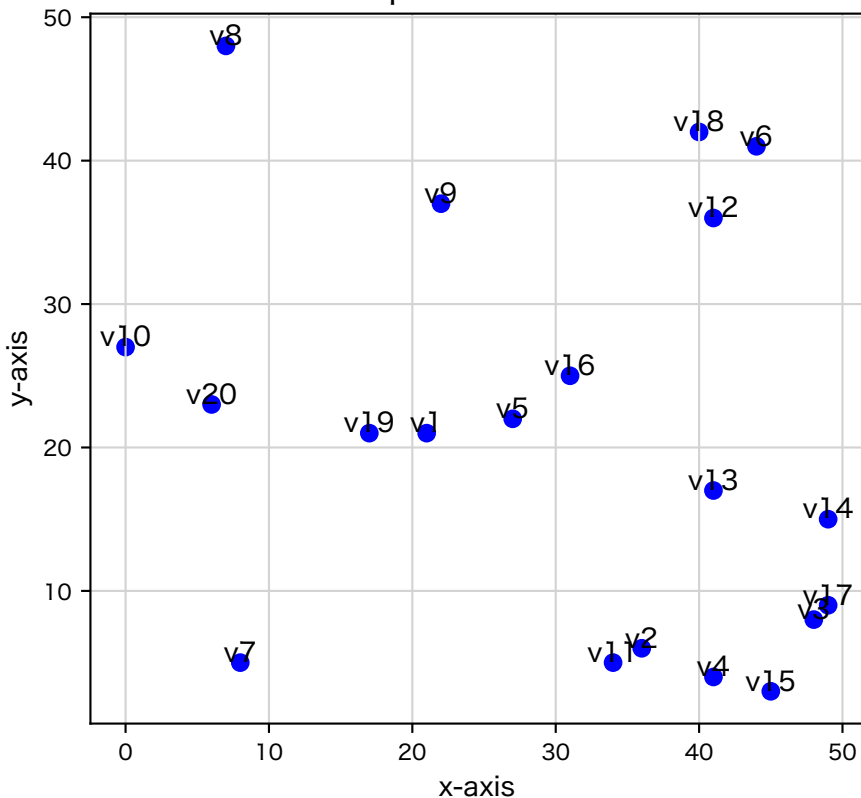
20 random points in a 50×50 Grid
