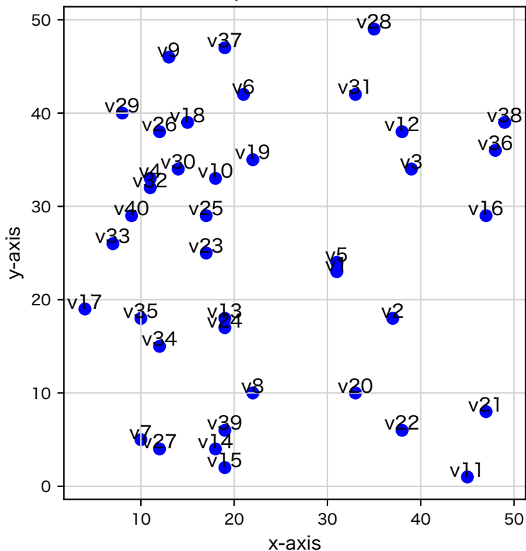
40 random points in a 50×50 Grid
