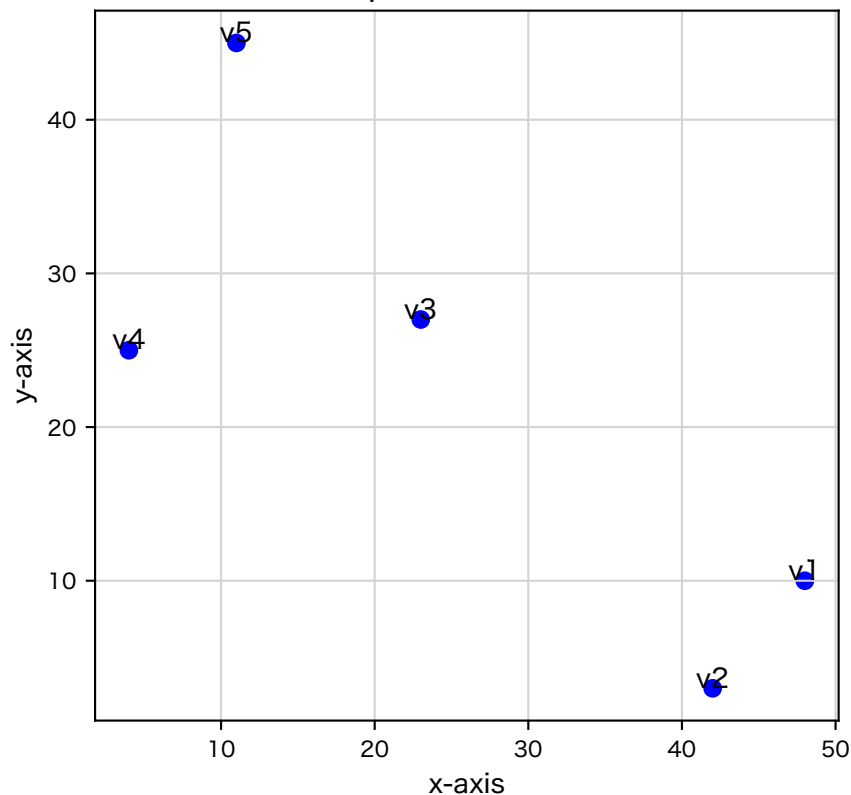
5 random points in a 50×50 Grid
