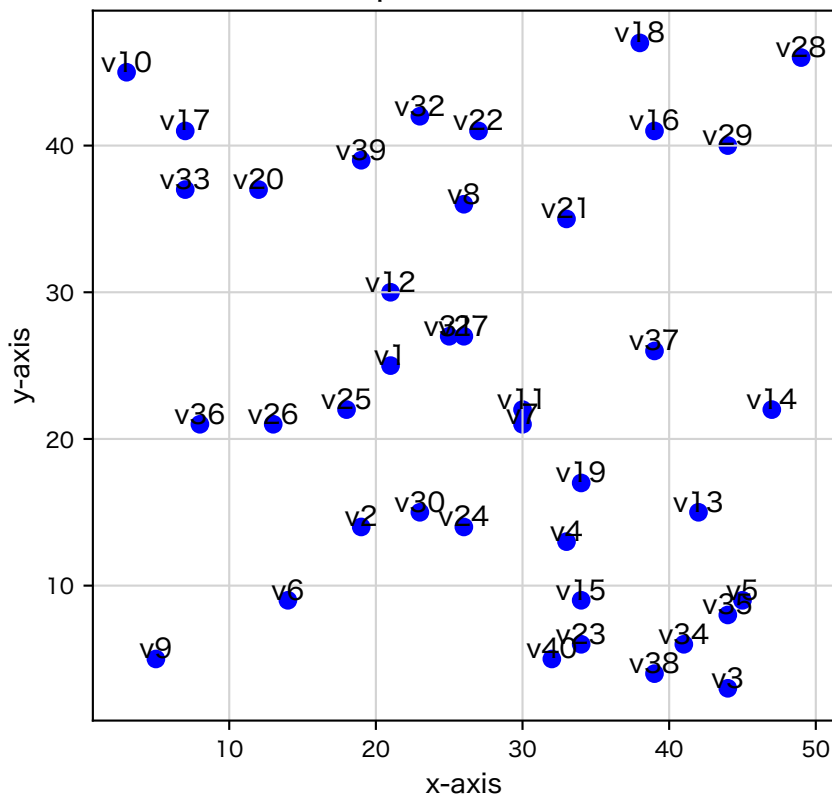
40 random points in a 50×50 Grid
