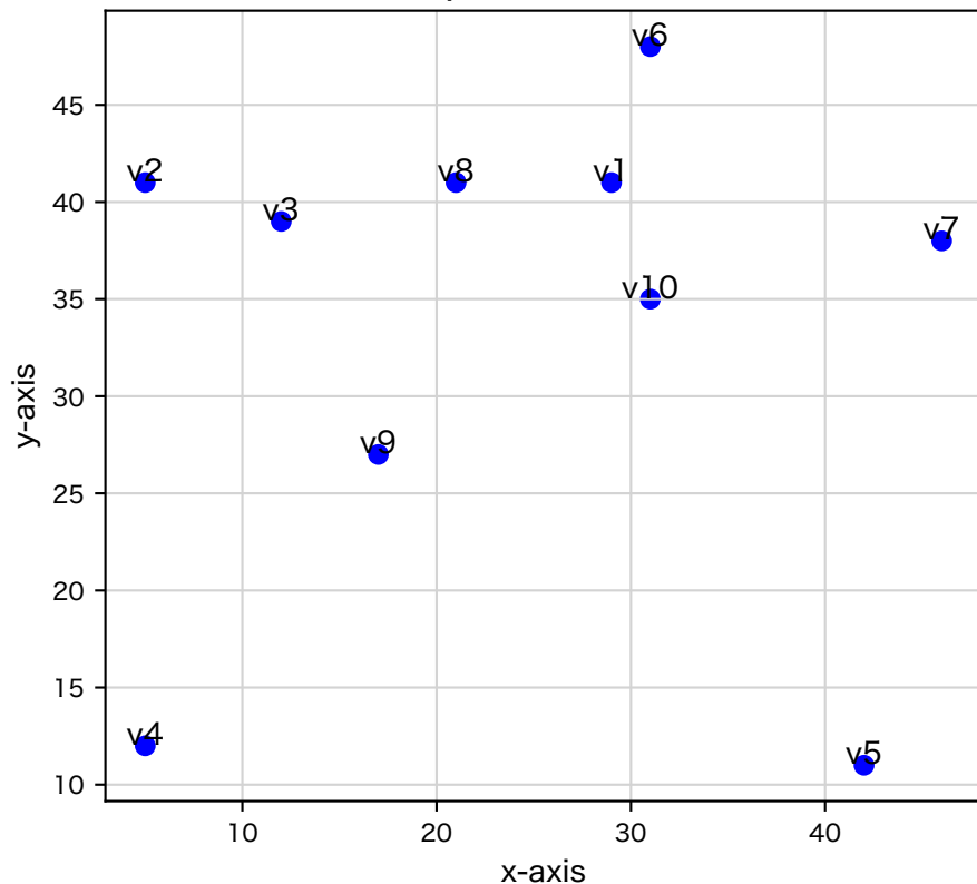
10 random points in a 50×50 Grid
