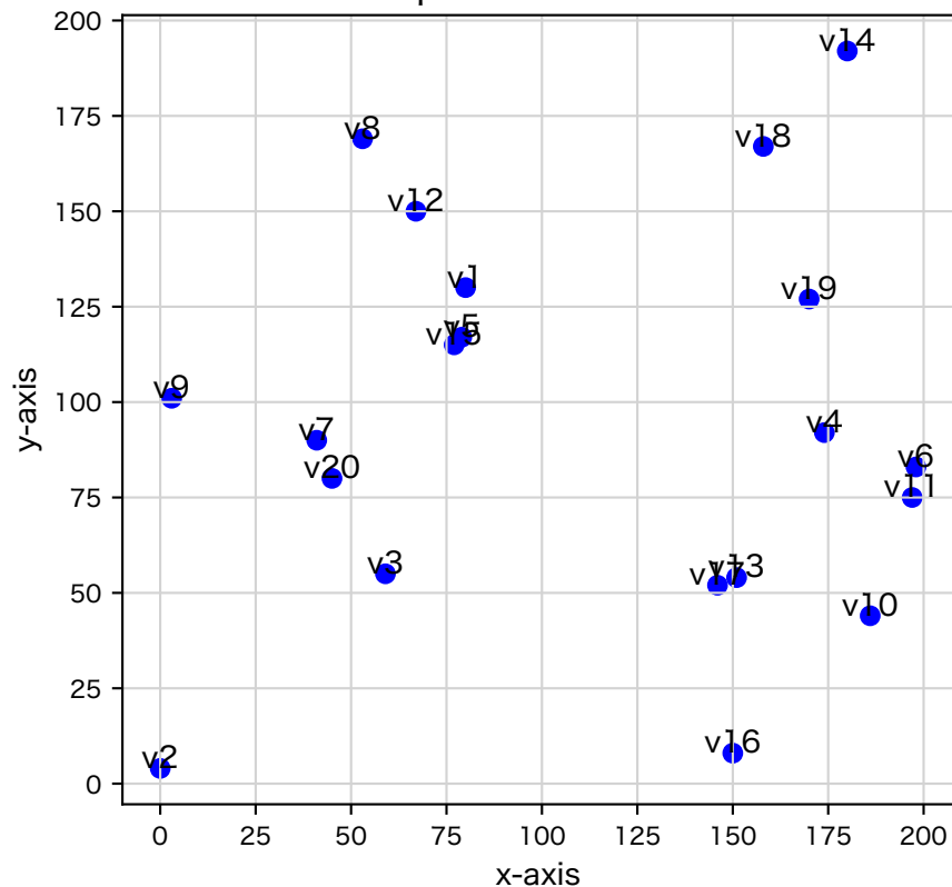
20 random points in a 200×200 Grid
