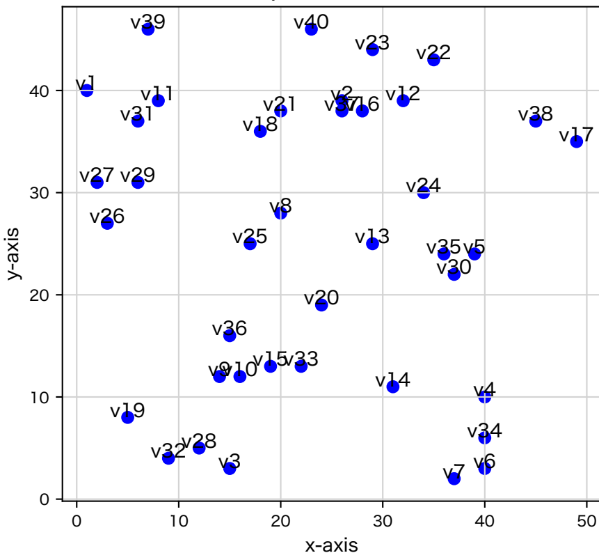
40 random points in a 50×50 Grid
