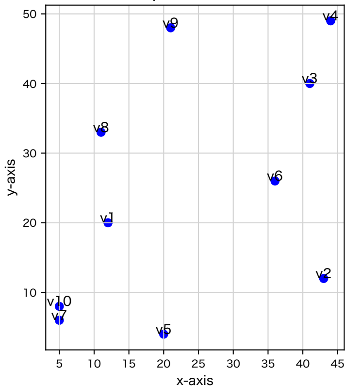
10 random points in a 50×50 Grid
