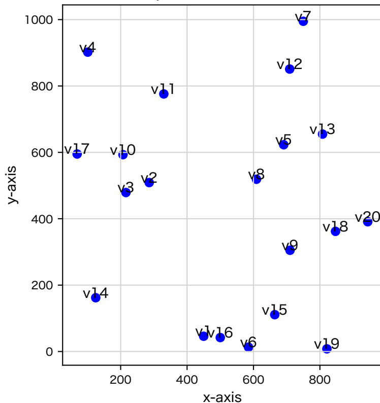
20 random points in a 1000×1000 Grid
