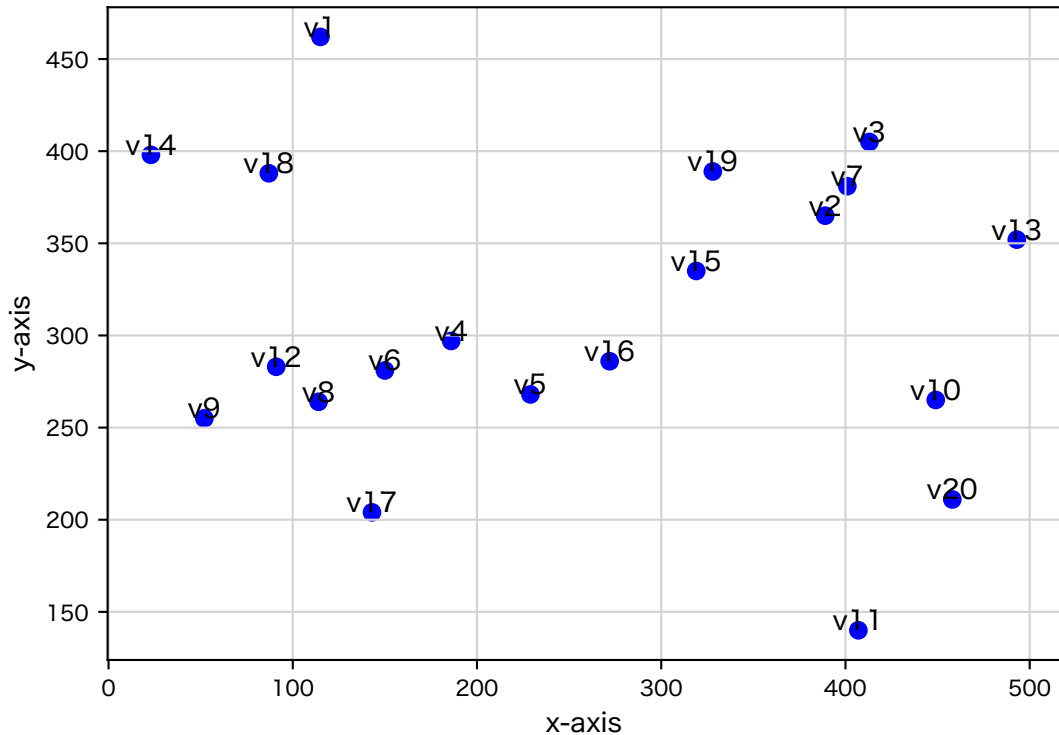
20 random points in a 500×500 Grid
