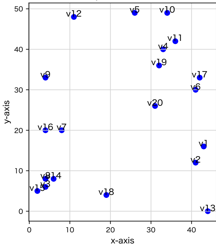
20 random points in a 50×50 Grid
