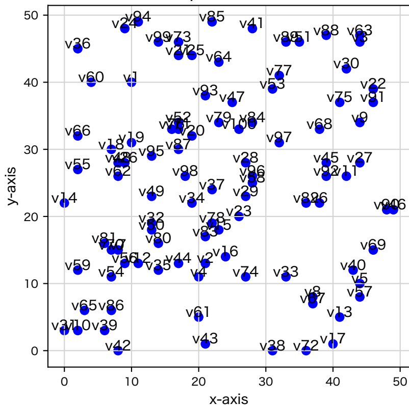
100 random points in a 50x50 Grid
