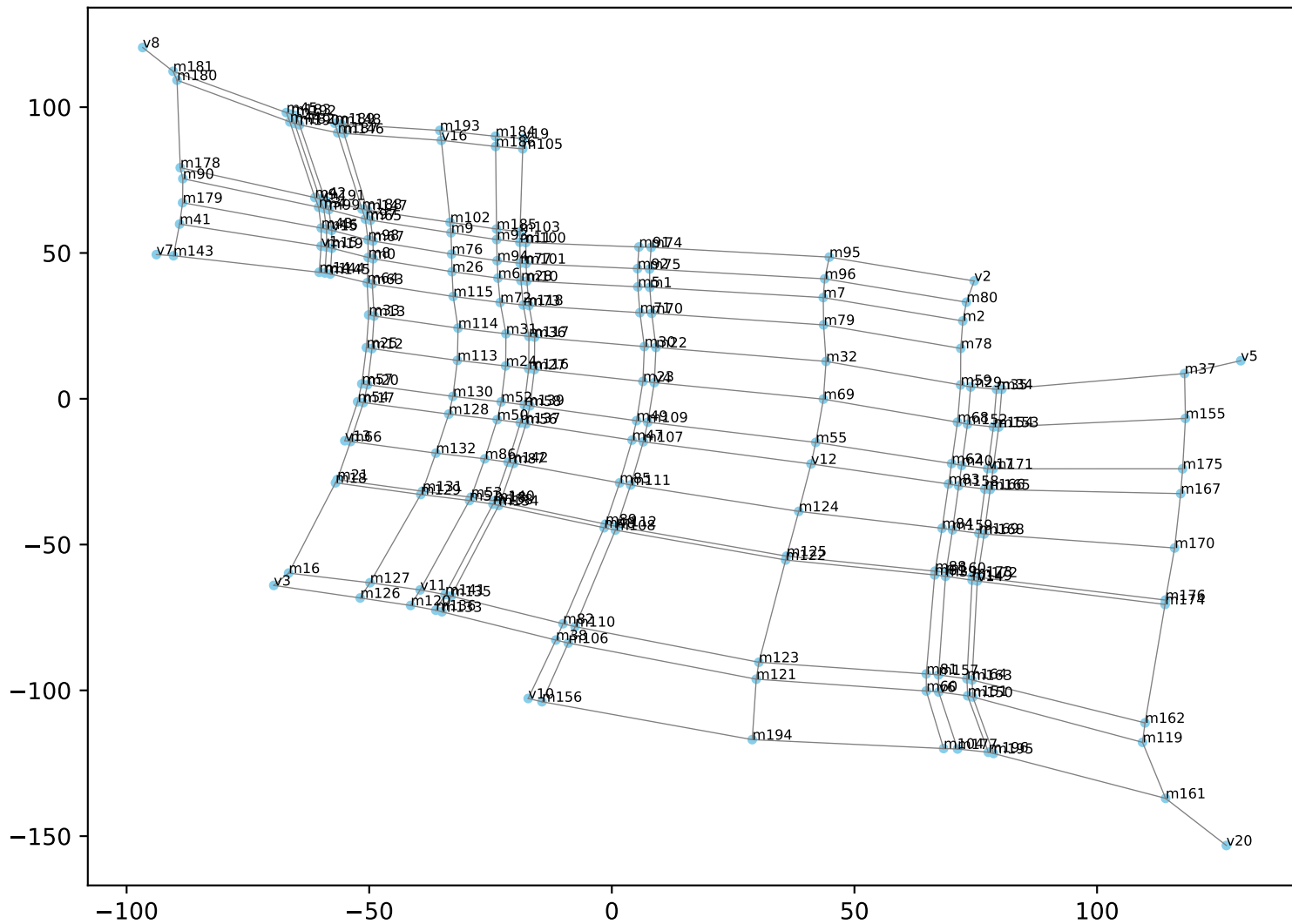
LG-graph with Weighted Edges (MDS)
