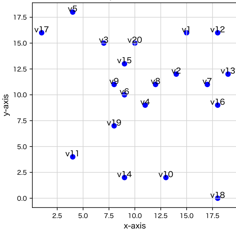
20 random points in a 20×20 Grid
