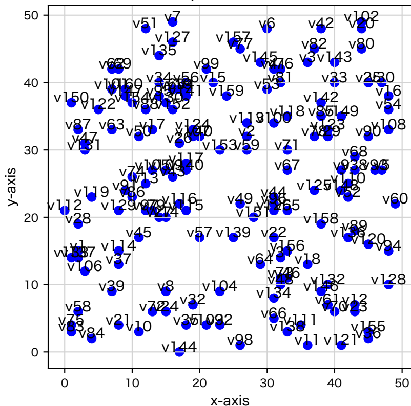
160 random points in a 50×50 Grid
