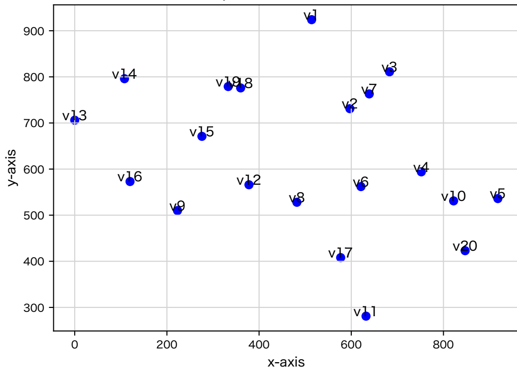
20 random points in a 1000×1000 Grid
