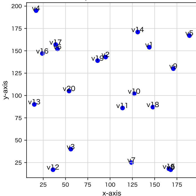
20 random points in a 200×200 Grid
