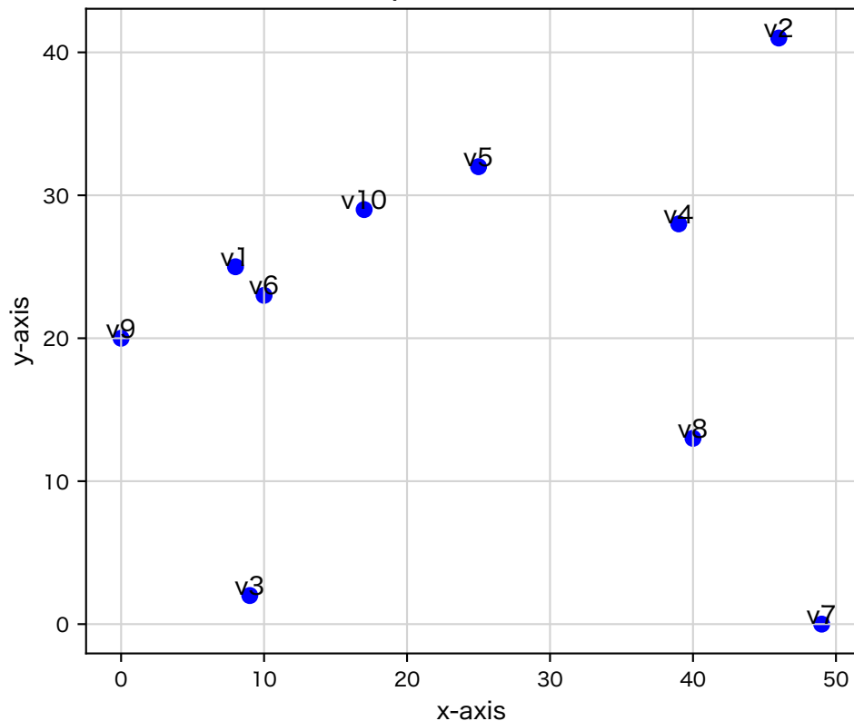
10 random points in a 50×50 Grid
