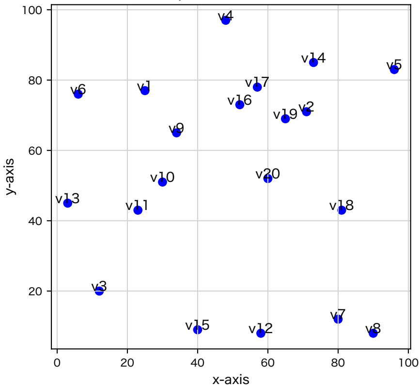
20 random points in a 100×100 Grid
