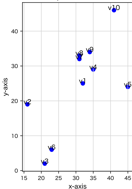
10 random points in a 50×50 Grid
