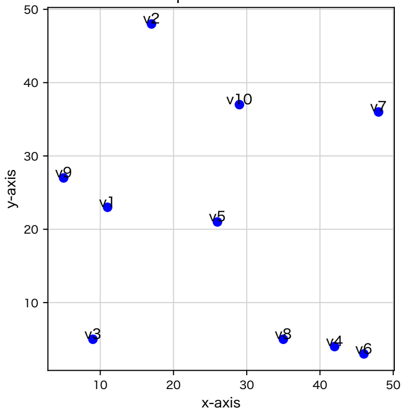
10 random points in a 50×50 Grid
