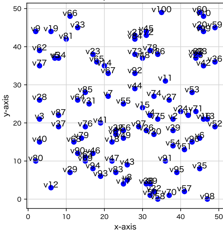
100 random points in a 50×50 Grid
