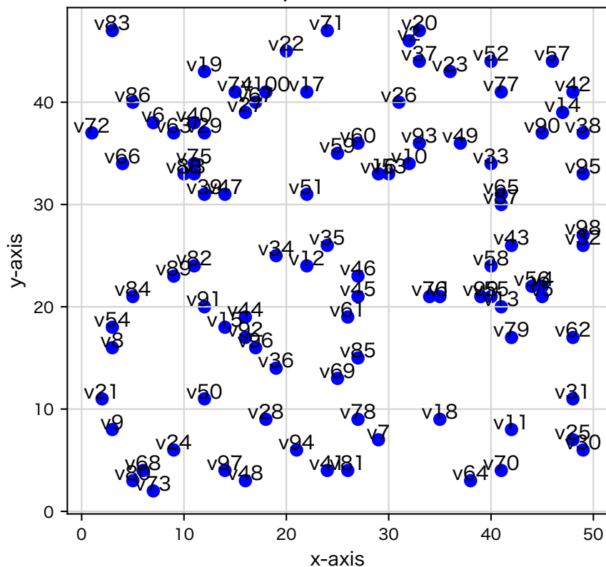
100 random points in a 50×50 Grid
