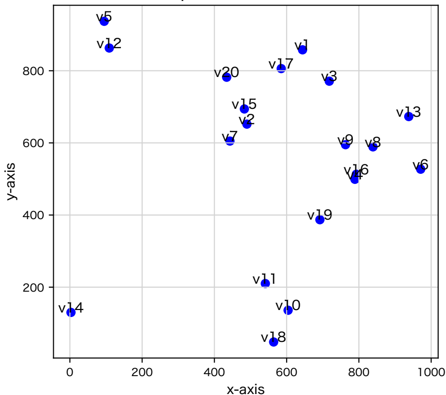
20 random points in a 1000×1000 Grid
