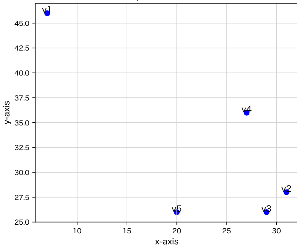
5 random points in a 50×50 Grid
