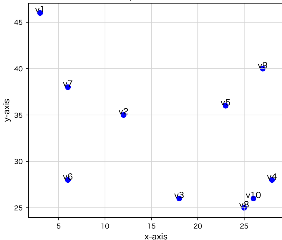
10 random points in a 50×50 Grid
