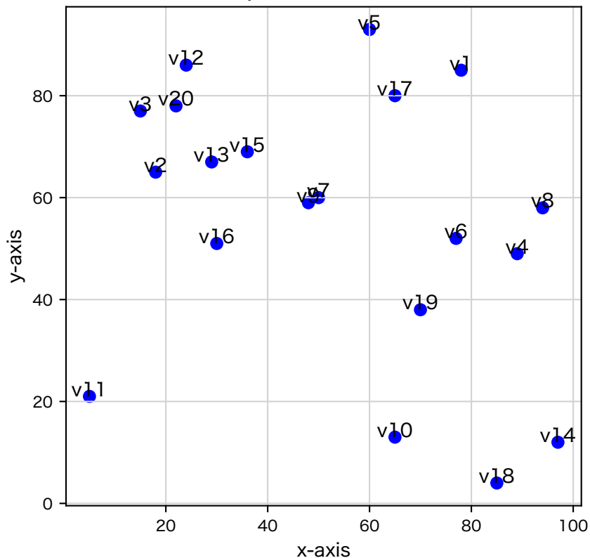
20 random points in a 100×100 Grid
