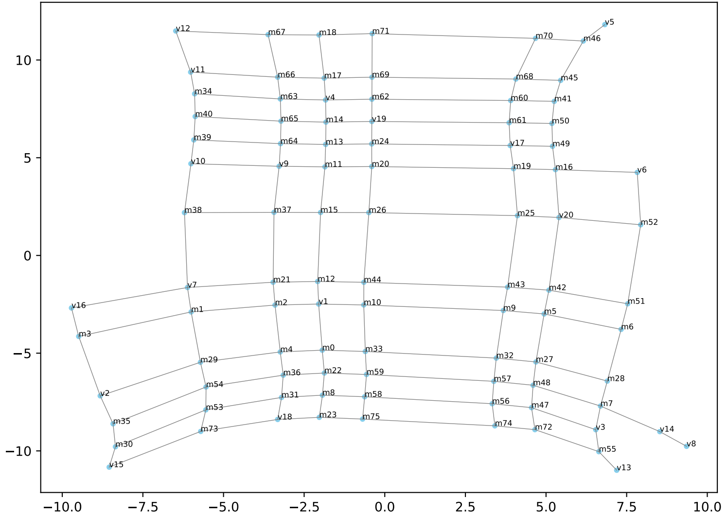
LG-graph with Weighted Edges (MDS)
