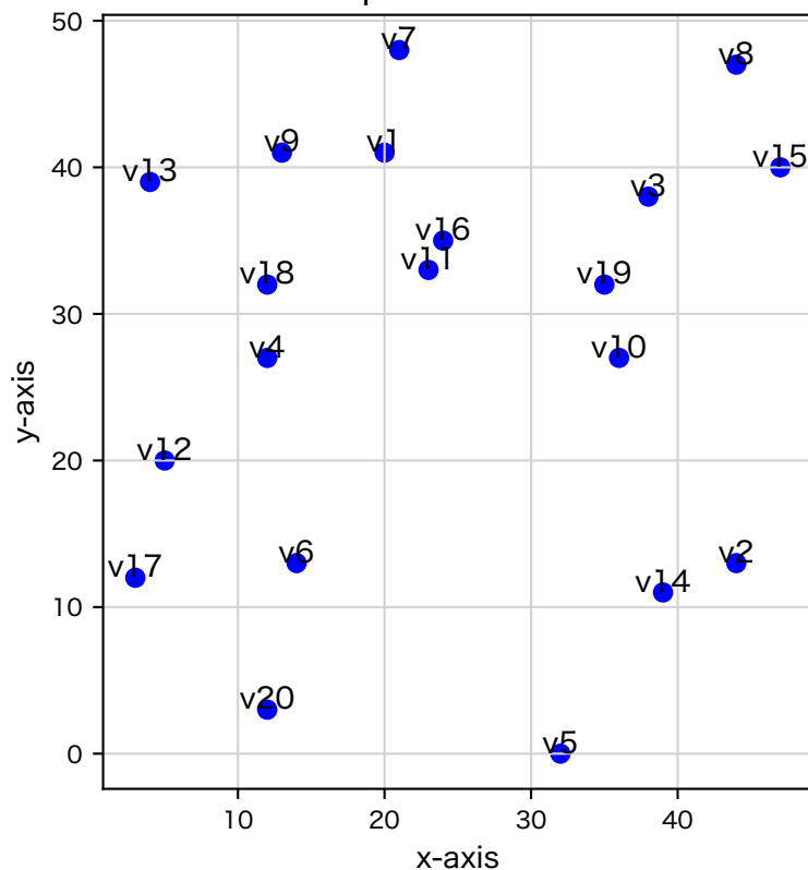
20 random points in a 50×50 Grid
