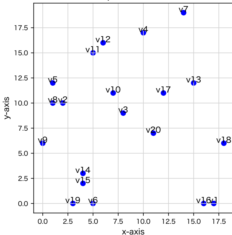
20 random points in a 20×20 Grid
