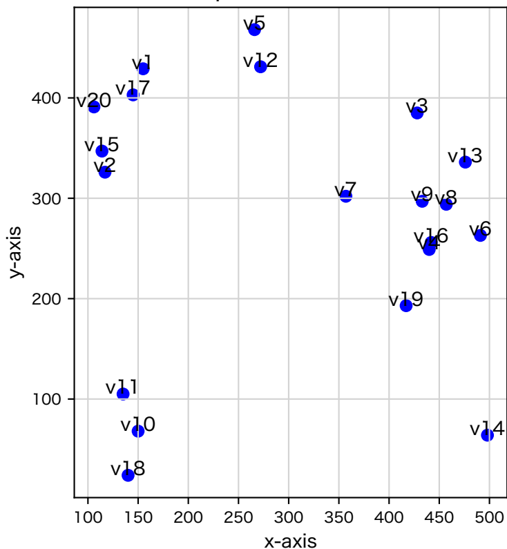
20 random points in a 500×500 Grid
