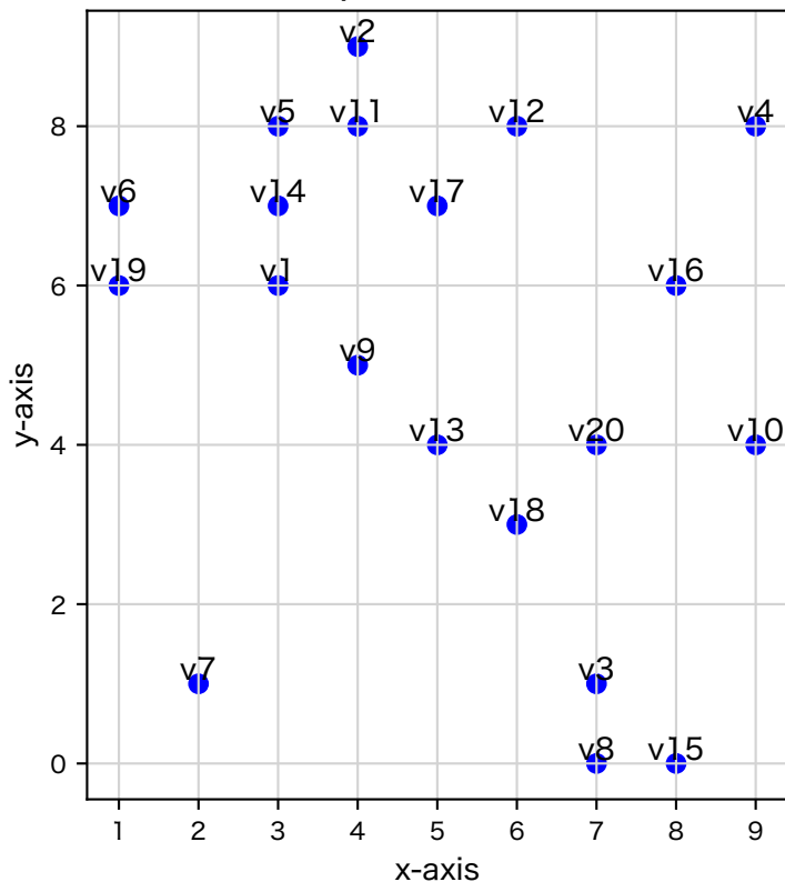
20 random points in a 10×10 Grid
