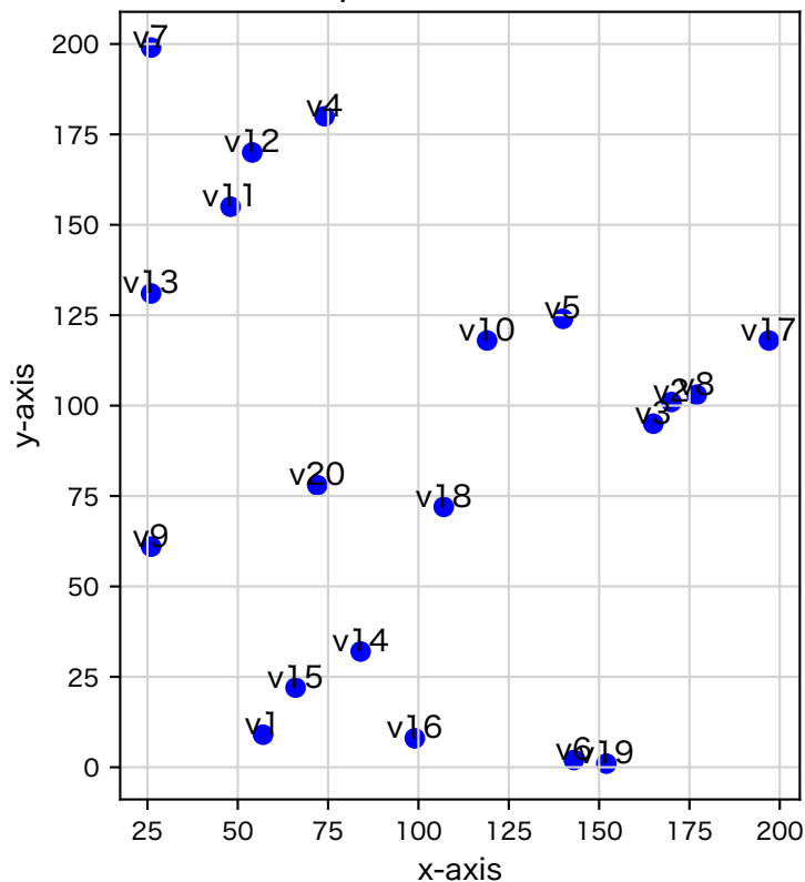
20 random points in a 200×200 Grid
