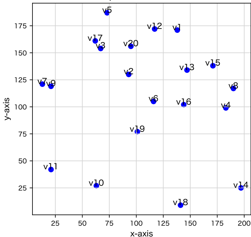
20 random points in a 200×200 Grid
