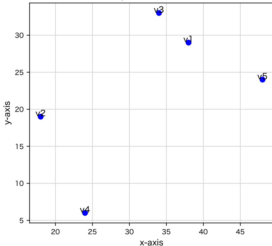
5 random points in a 50×50 Grid
