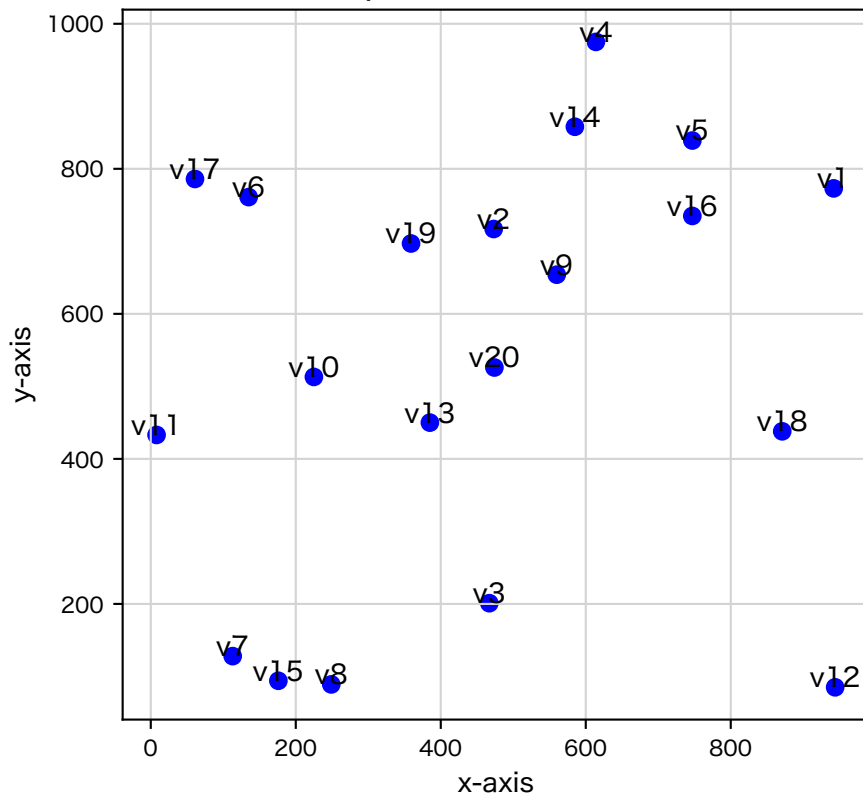
20 random points in a 1000×1000 Grid
