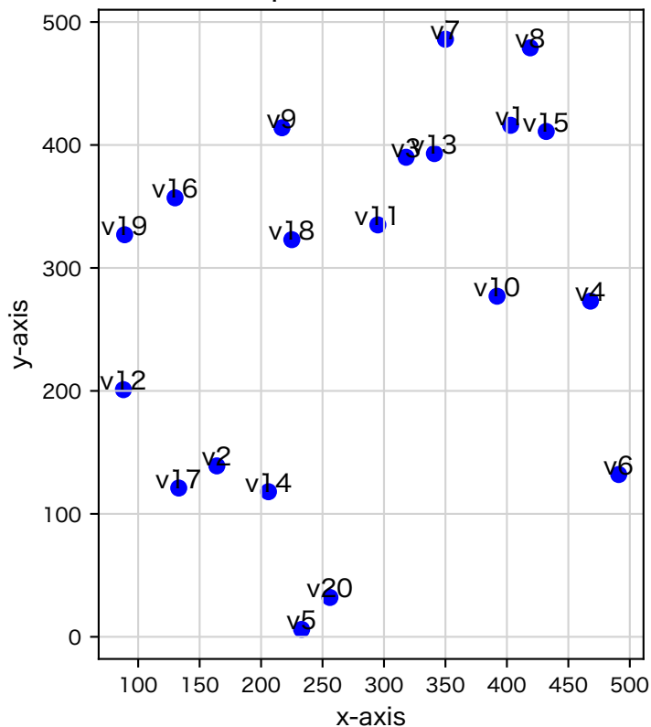
20 random points in a 500×500 Grid
