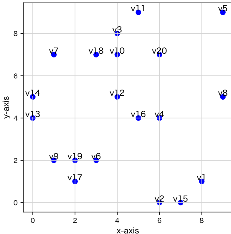
20 random points in a 10×10 Grid
