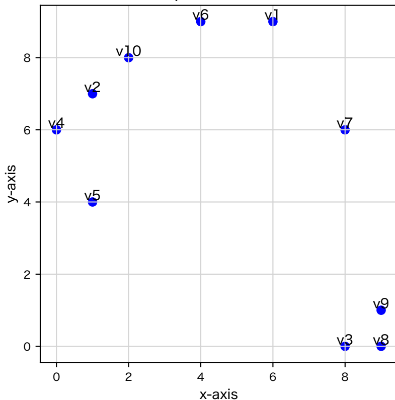
10 random points in a 10×10 Grid
