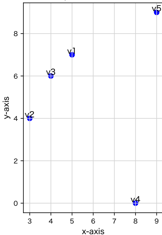
5 random points in a 10×10 Grid
