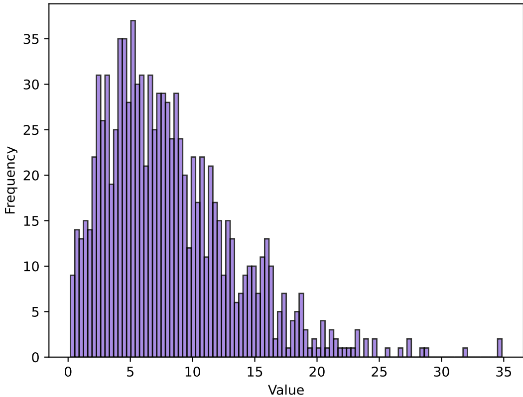
1000 Random Variates: Noncentral Chi-Square (df=3, nonc=5)
