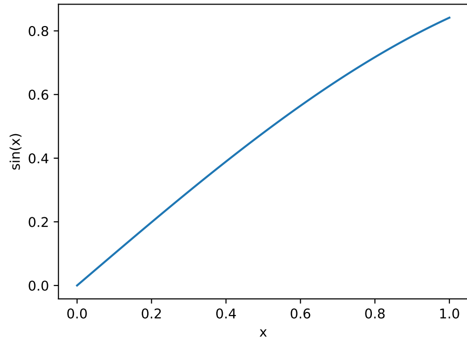
\sin(x)
