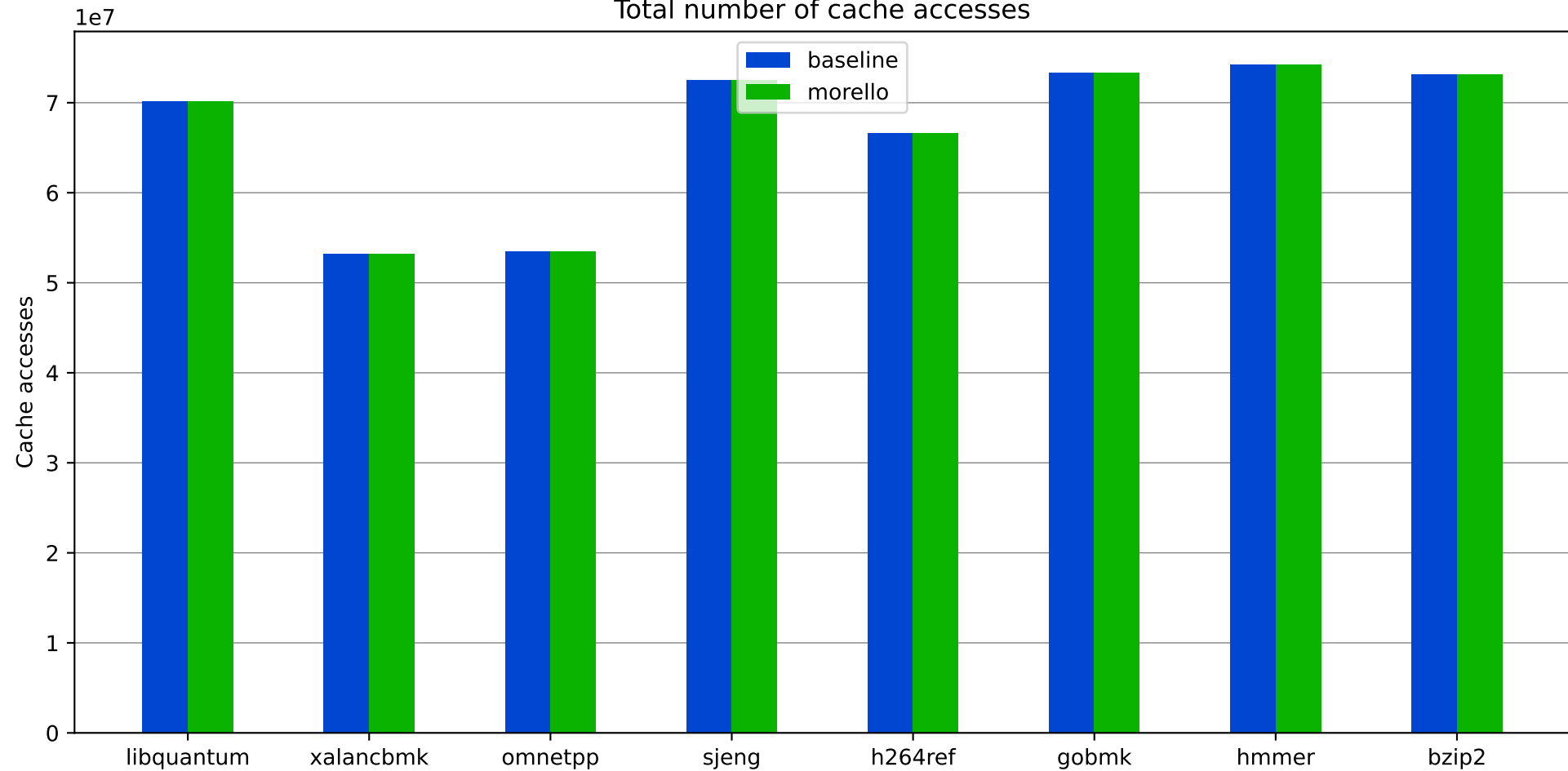
Total number of cache accesses
