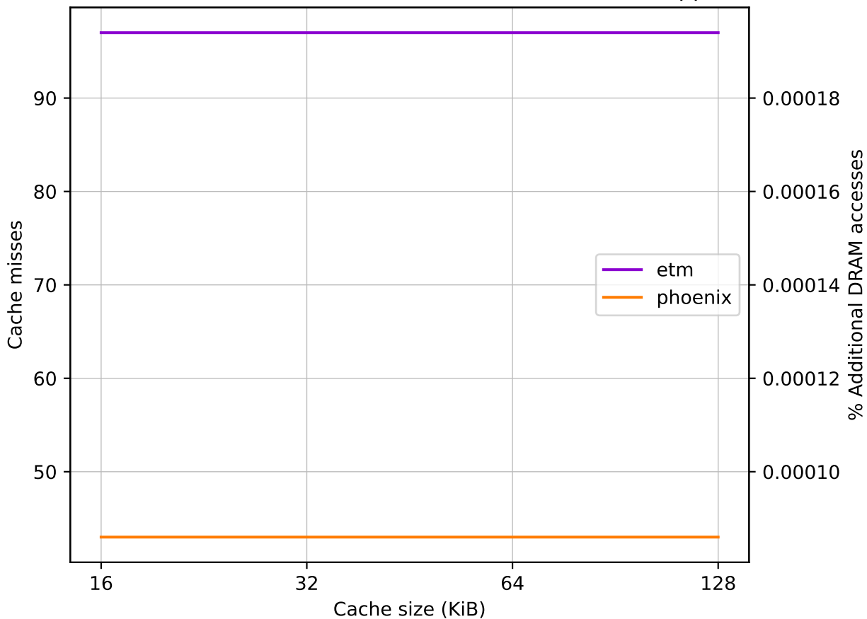
Total number of cache misses for workload omnetpp
