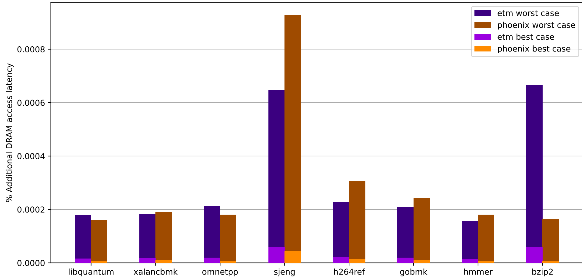
Best and worst case additional DRAM access latency
